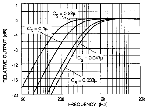
Fig. 5. Closed Loop Frequency Response with Various C_S Values
