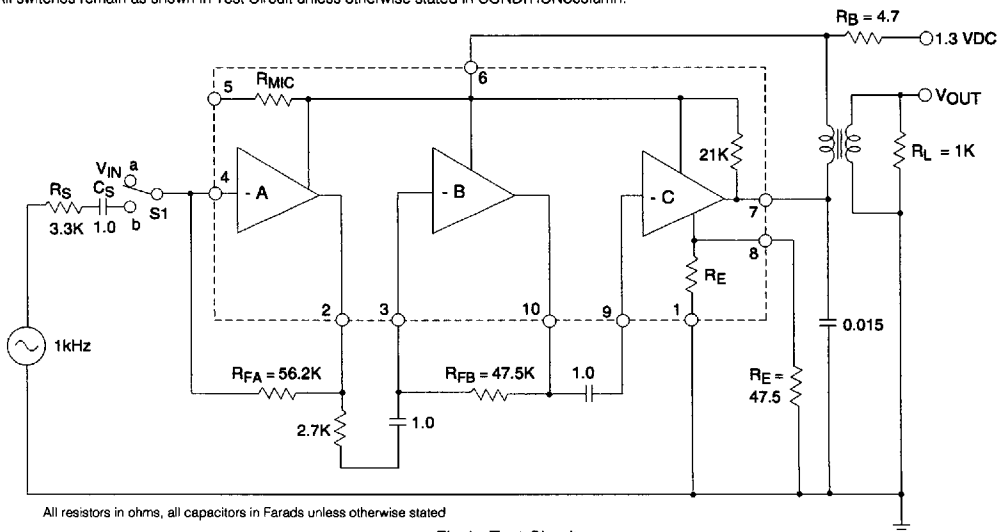
Fig.1 Test Circuit
