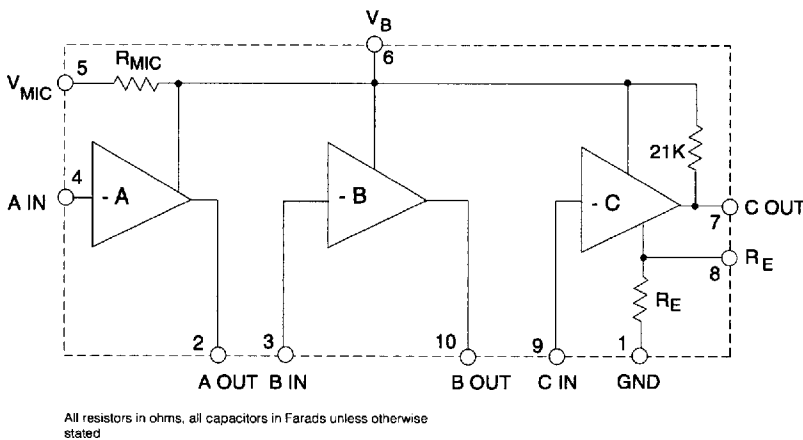
BLOCK DIAGRAM
