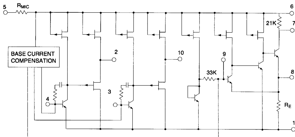
Fig. 2 Functional Schematic
