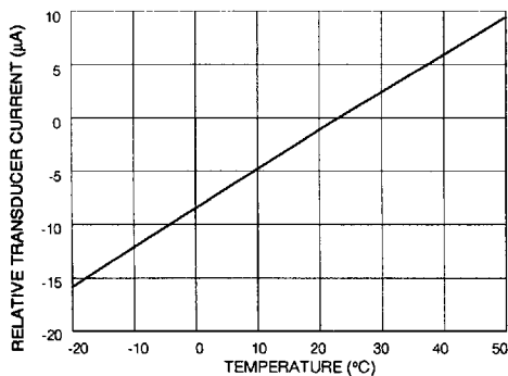
Fig. 8 Transducer Current vs Temperature
