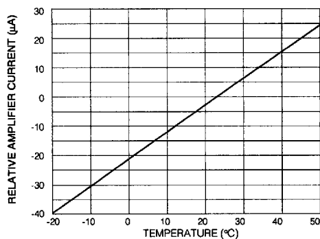
Fig. 9 Amplifier Current vs Temperature
