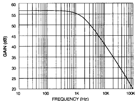
Fig. 7 Preamplifier Open Loop Frequency Response
