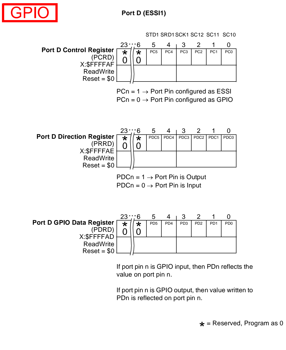
Figure B-27. Port D Registers (PCRD, PRRD, PDRD)
