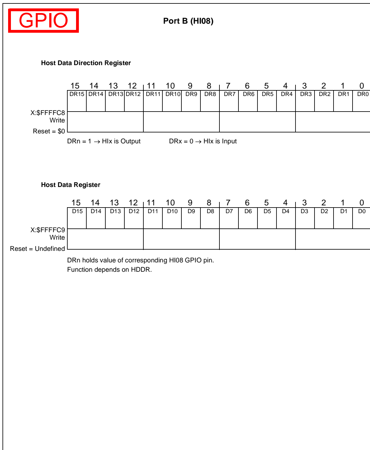
Figure B-25. Host Data Direction and Host Data Registers (HDDR, HDR)
