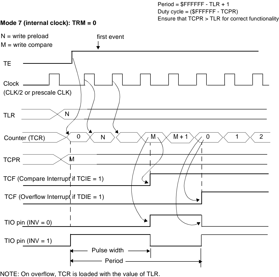
Figure 9-17. Pulse Width Modulation Toggle Mode, TRM = 0
