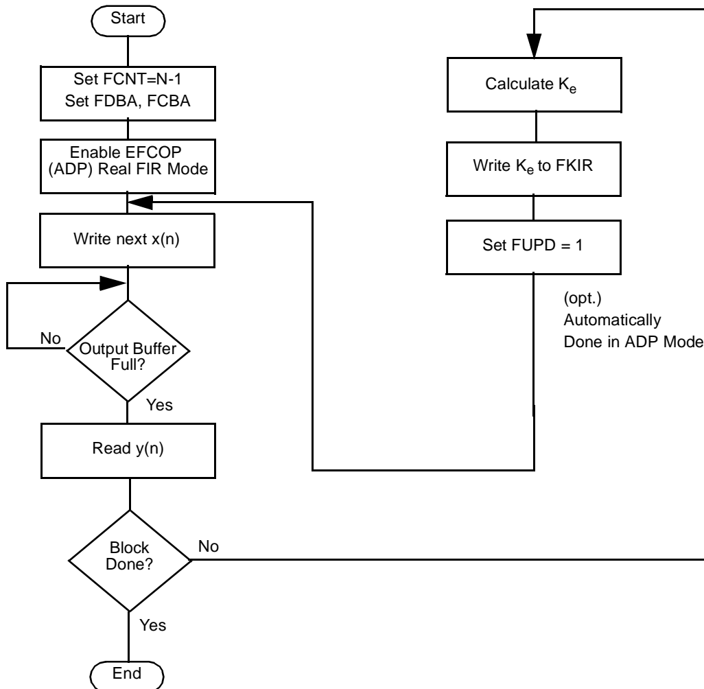
Figure 10-12. Adaptive FIR Filter Using Polling
