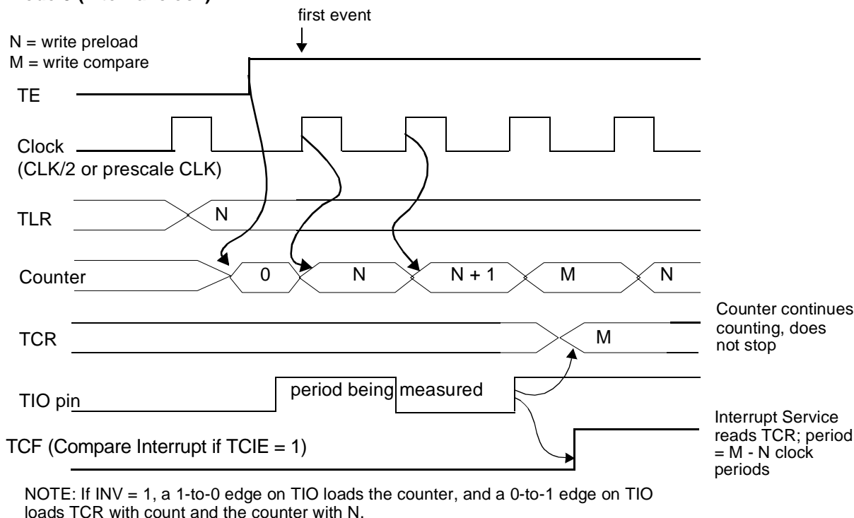
Figure 9-13. Period Measurement Mode, TRM = 1
