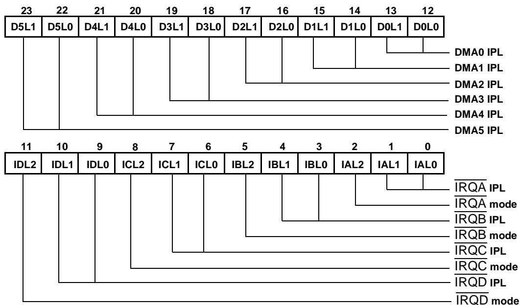
Figure 4-1. Interrupt Priority Register C (IPR-C) (X:$FFFFFF)
