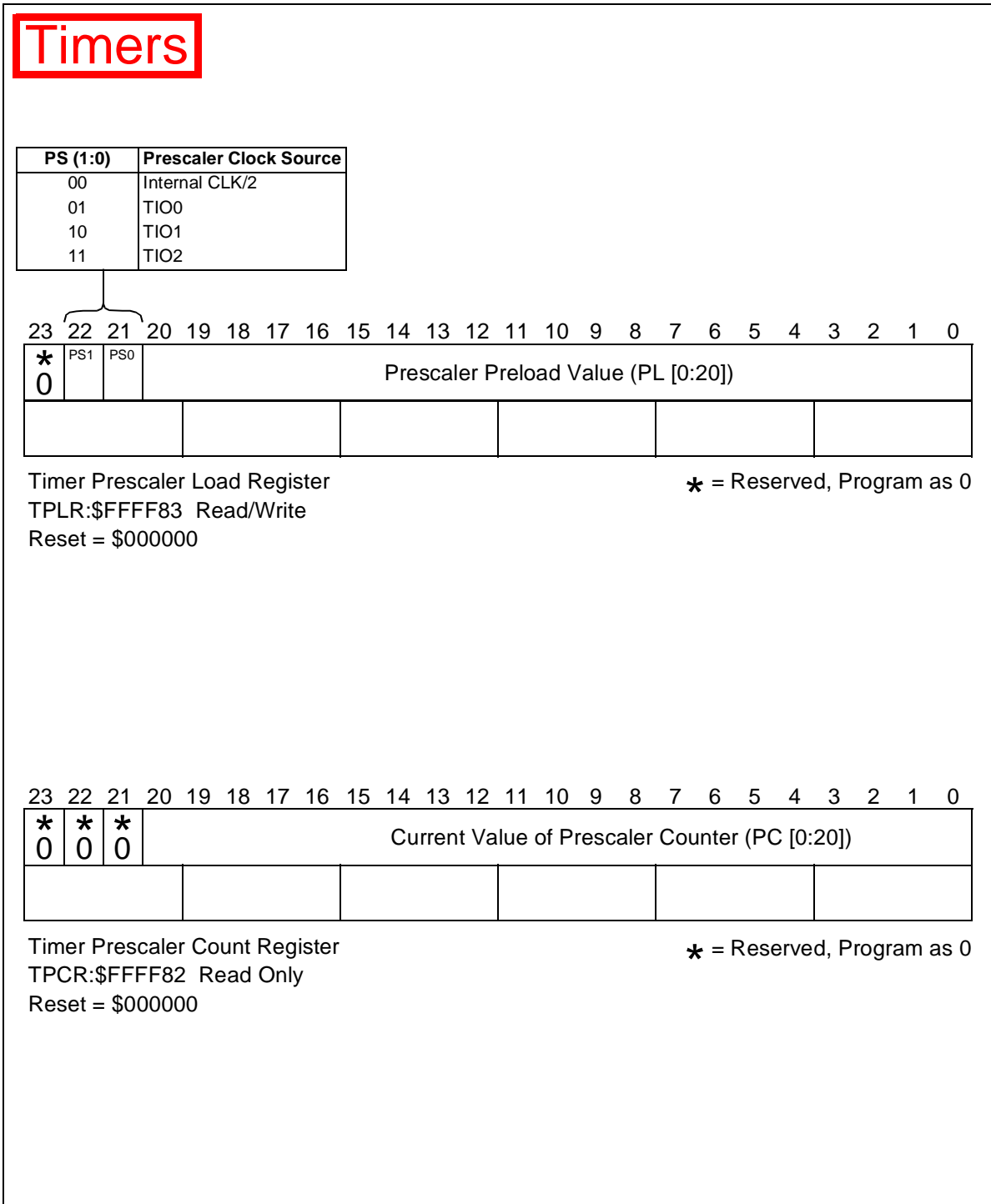
Figure B-22. Timer Prescaler Load/Count Register (TPLR, TPCR)
