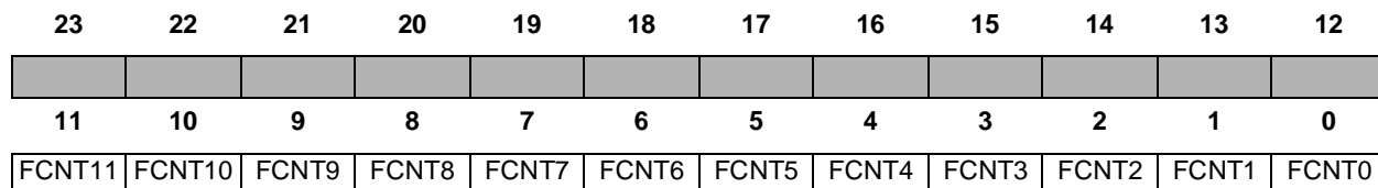
Figure 10-4. Filter Count (FCNT) Register
