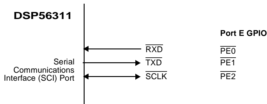
Figure 5-5. Port E Signals
