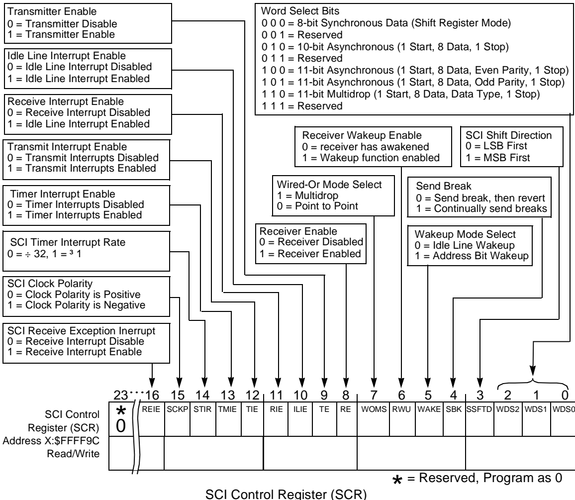
Figure B-19. SCI Control Register (SCR)
