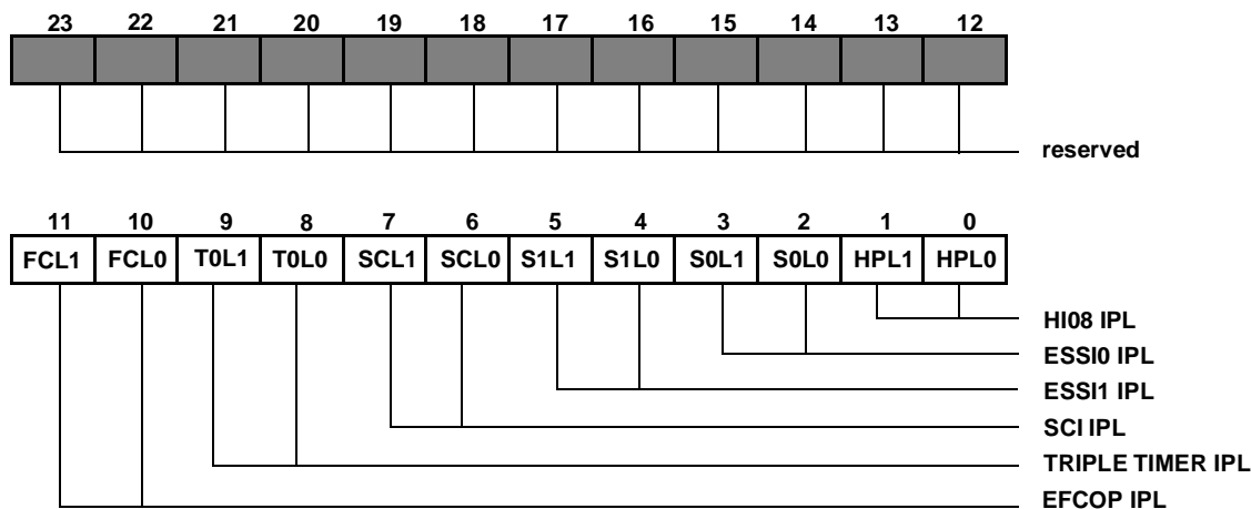
Figure 4-2. Interrupt Priority Register P (IPR-P) (X:$FFFFFE)
