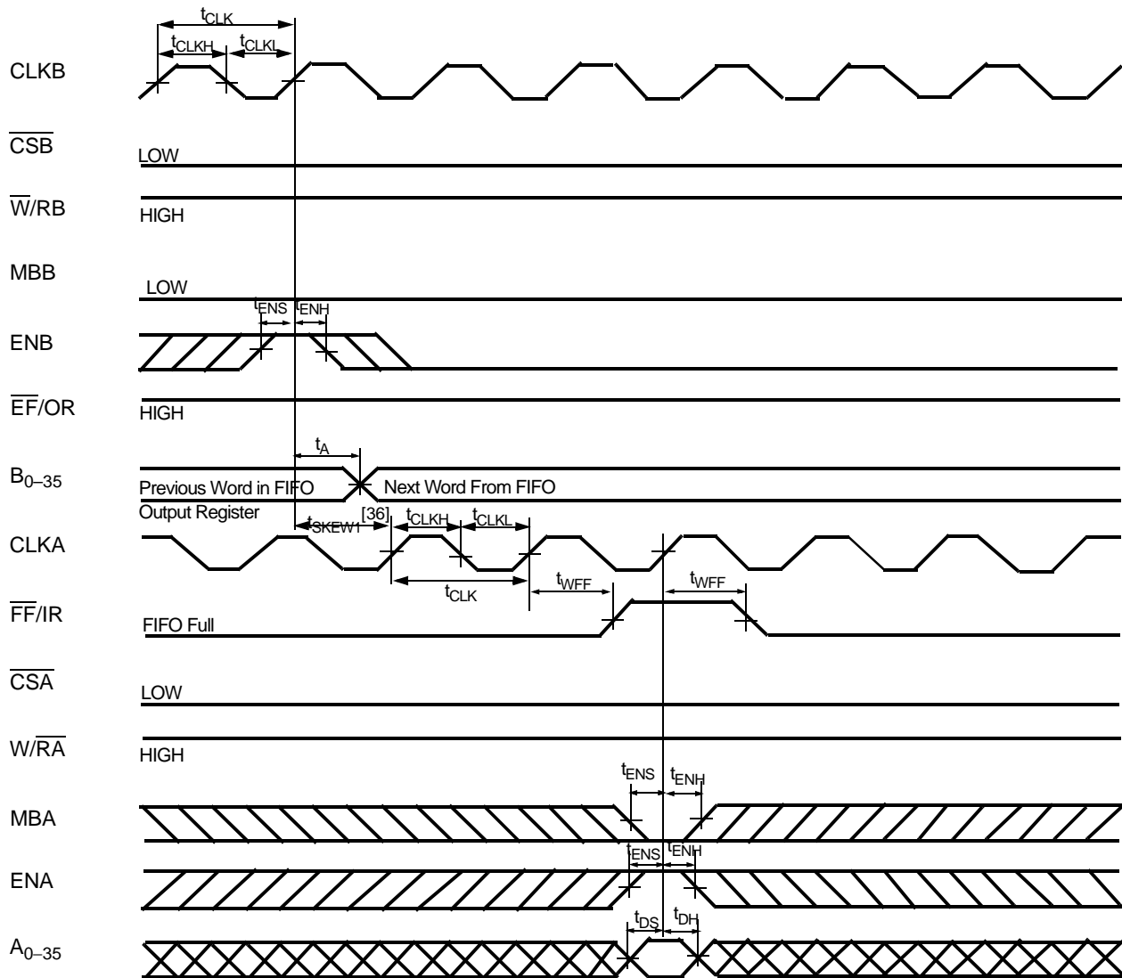
\overline{FF} Flag Timing and First Available Write when FIFO is Full (CY Standard Mode) [34]
