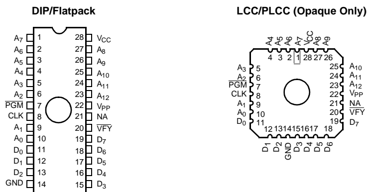
Figure 1. Programming Pinout
