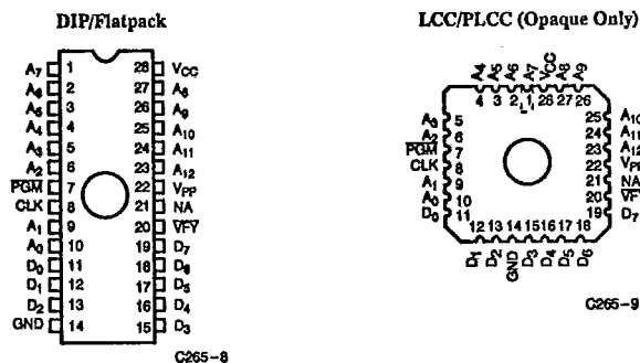
Figure 1. Programming Pinout
