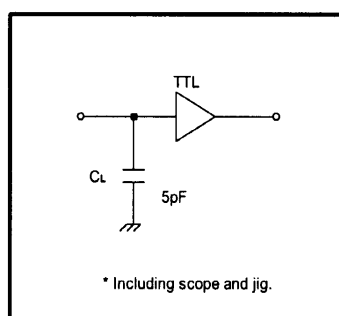
Figure 2. Output Load for t_{CLZ1} , t_{CLZ2} , t_{OHZ} , t_{OLZ} , t_{CHZ1} , t_{CHZ2} , t_{WHZ} , and t_{OW}
