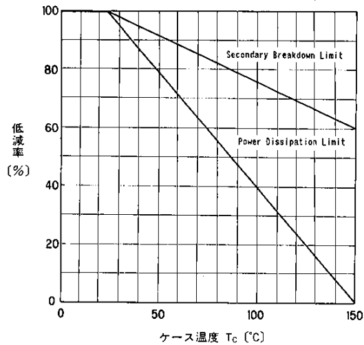
ASO Derating
