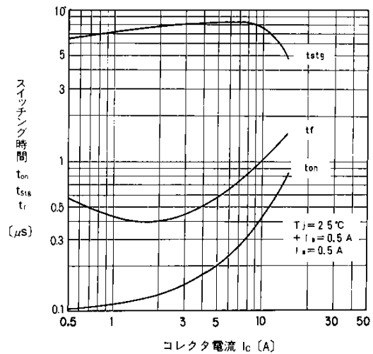
Switching Time
