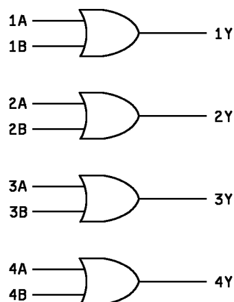
FIGURE 3. Logic diagram.
