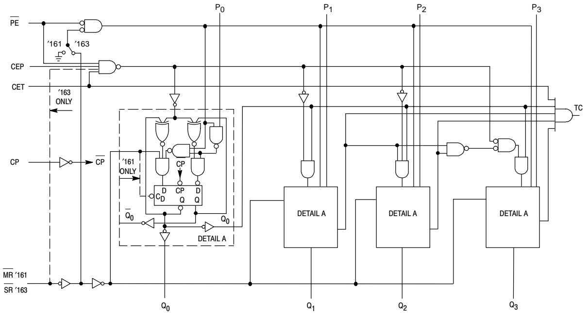
Figure 4. Logic Diagram
