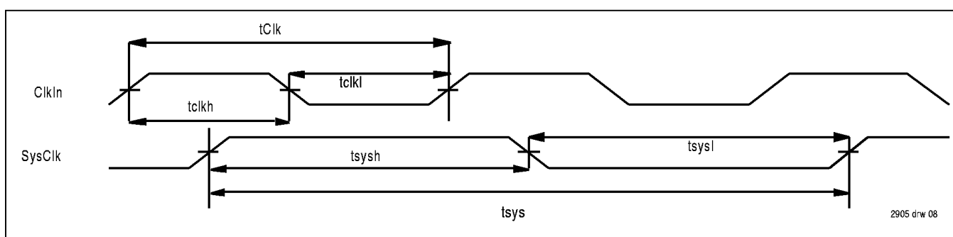
Figure 2: Clocking Sequence
