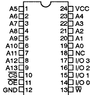
Pinout 24 pins (top view)
