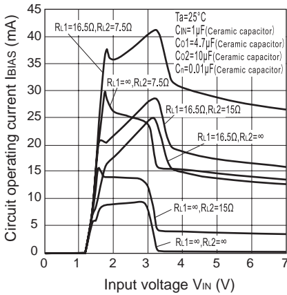
Fig.8 Circuit Operating Current vs. Input Voltage (PQ2L3152MSPQ)(Typical Value)
