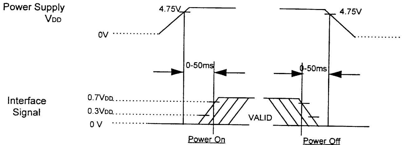
Power ON/OFF Sequence
