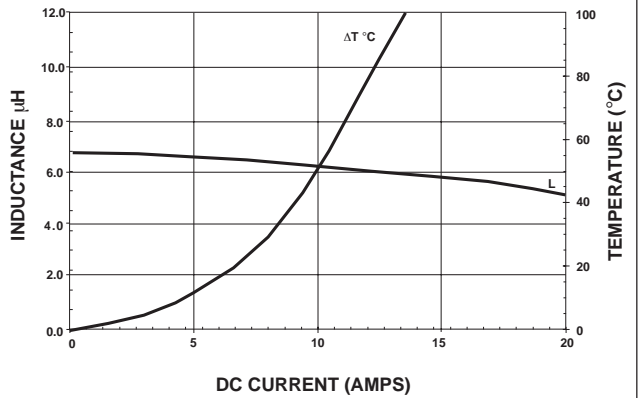
IHLP-5050CE-01 6.8 \mu H
