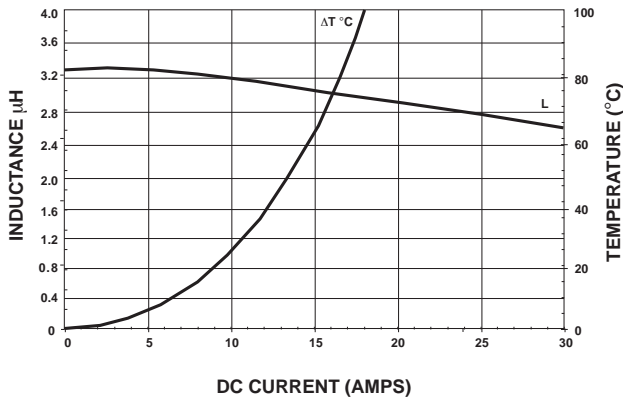
IHLP-5050CE-01 3.3 \mu H
