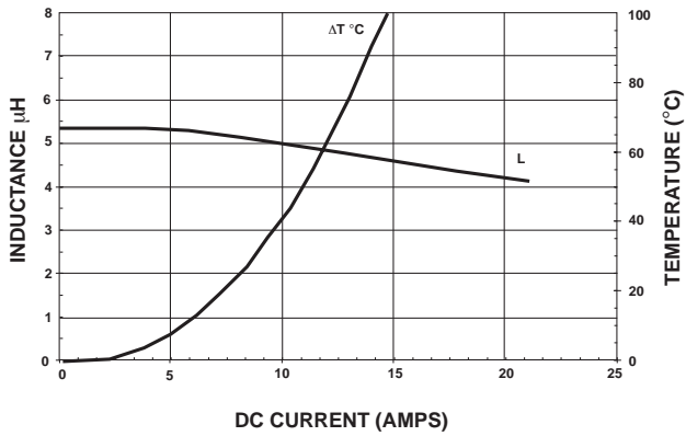
IHLP-5050CE-01 5.6 \mu H
