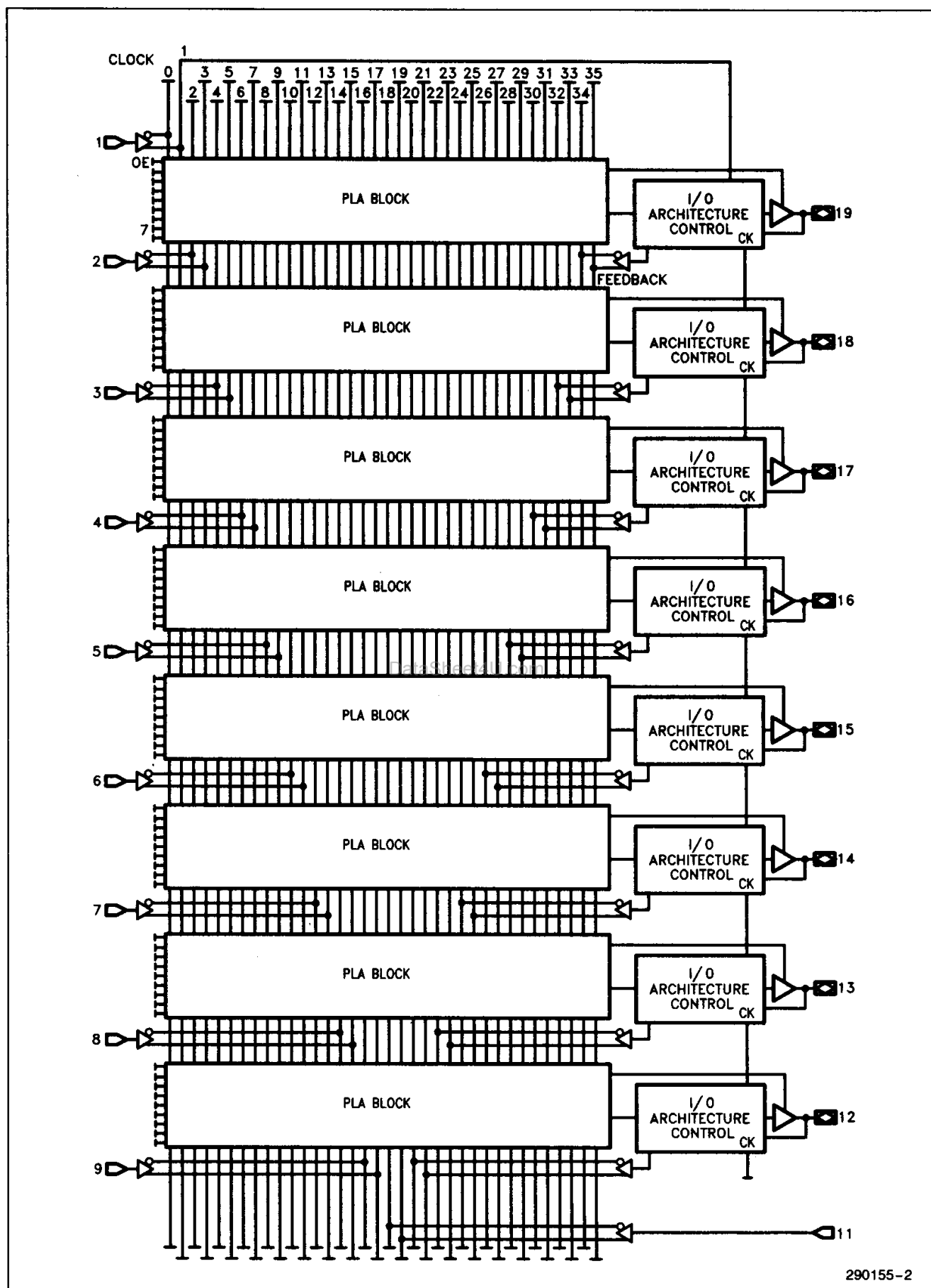
Figure 1. 5C032 Architecture
