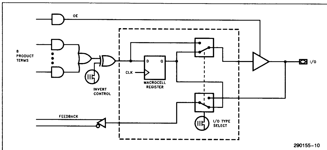
Figure 3. 5C032 I/O Architecture Control
