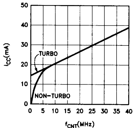
Current in Relation to Frequency
