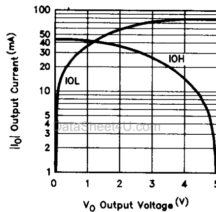
Output Drive Current in Relation to Voltage
