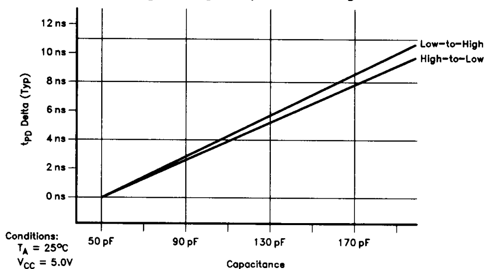
t_{PD} Derating vs Capacitive Loading
