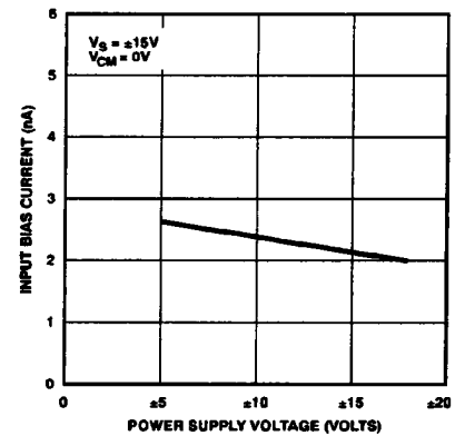
Figure 11. Input Bias Current vs. Supply Voltage
