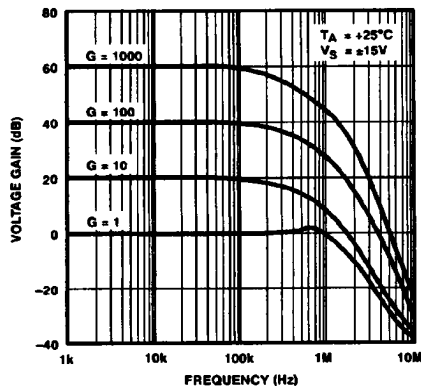
Figure 12. Closed-Loop Voltage Gain vs. Frequency
