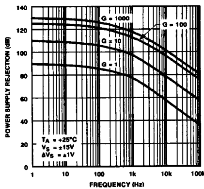
Figure 15. Positive PSR vs. Frequency
