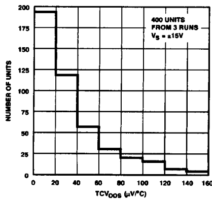
Figure 7. Typical Distribution of TCV_{OOS}
