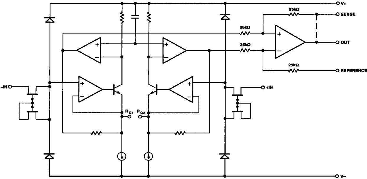
Figure 2. Simplified Schematic
