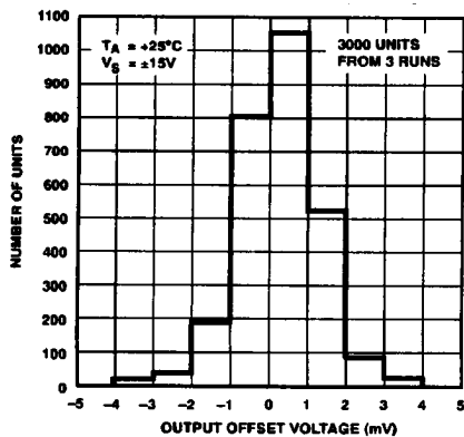
Figure 6. Typical Distribution of Output Offset Voltage
