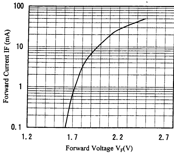
Forward Current vs. Forward Voltage ( T_a=25^\circ\text{C} )
