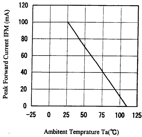
Peak Forward Current Derating Curve
