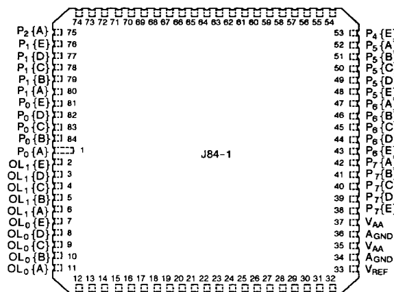
PLCC TOP VIEW
