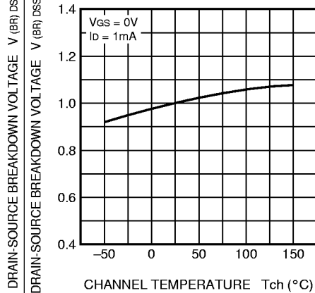
BREAKDOWN VOLTAGE VS. CHANNEL TEMPERATURE (TYPICAL)
