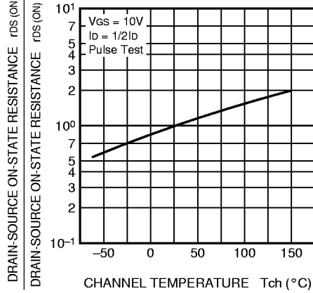
ON-STATE RESISTANCE VS. CHANNEL TEMPERATURE (TYPICAL)
