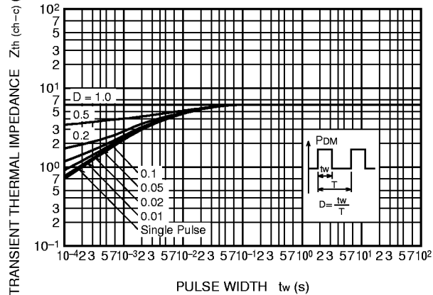
TRANSIENT THERMAL IMPEDANCE CHARACTERISTICS
