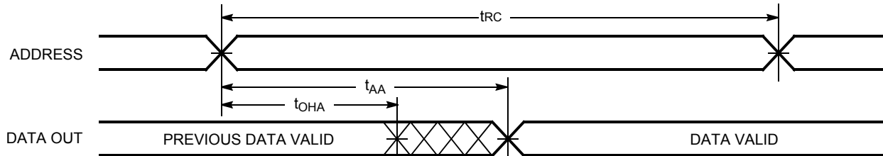
Read Cycle No. 2 ( \overline{\text{OE}} Controlled) [17, 18]
