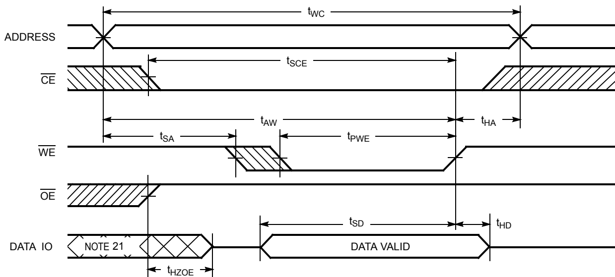
Write Cycle No. 1 ( \overline{\text{WE}} Controlled, \overline{\text{OE}} HIGH During Write) [19, 20]
