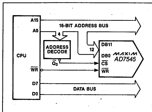
Figure 10. Connecting the AD7545 to 8-Bit Processors via the Address Bus
