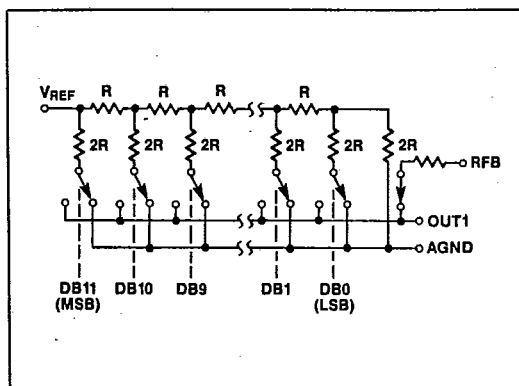
Figure 1. Simplified D/A Circuit of AD7545
