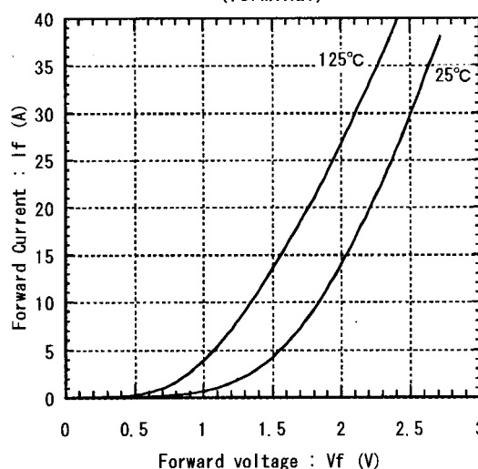
Forward current vs. Forward voltage (Terminal)
