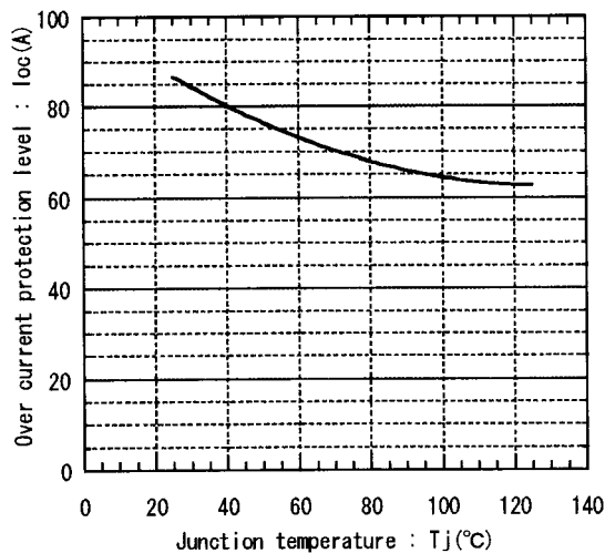
Over current protection vs. Junction temperature Vcc=15V
