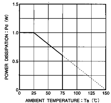
Fig.8 Power dissipation curve
