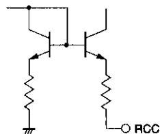
(9) Torque ripple (RCC : 19 pin)
