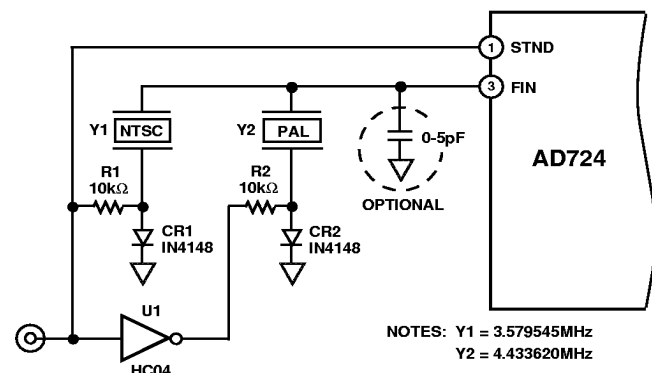
Figure 17. Crystal Selection Circuit
