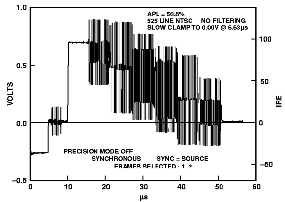
Figure 4. 100% Color Bars, NTSC
