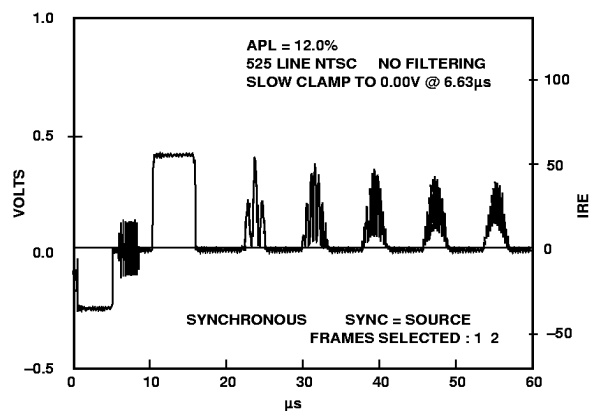
Figure 8. Multipulse, NTSC
