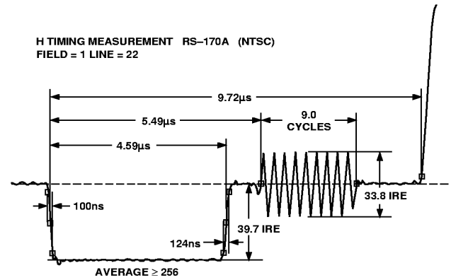
Figure 12. Horizontal Timing, NTSC
