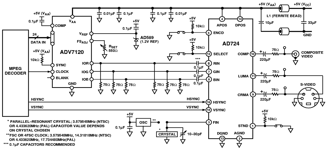
Figure 16. AD724 and ADV7120/ADV7122 Providing MPEG Video Solution
