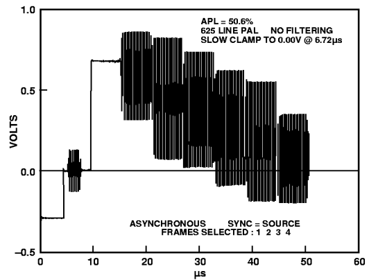
Figure 5. 100% Color Bars, PAL
