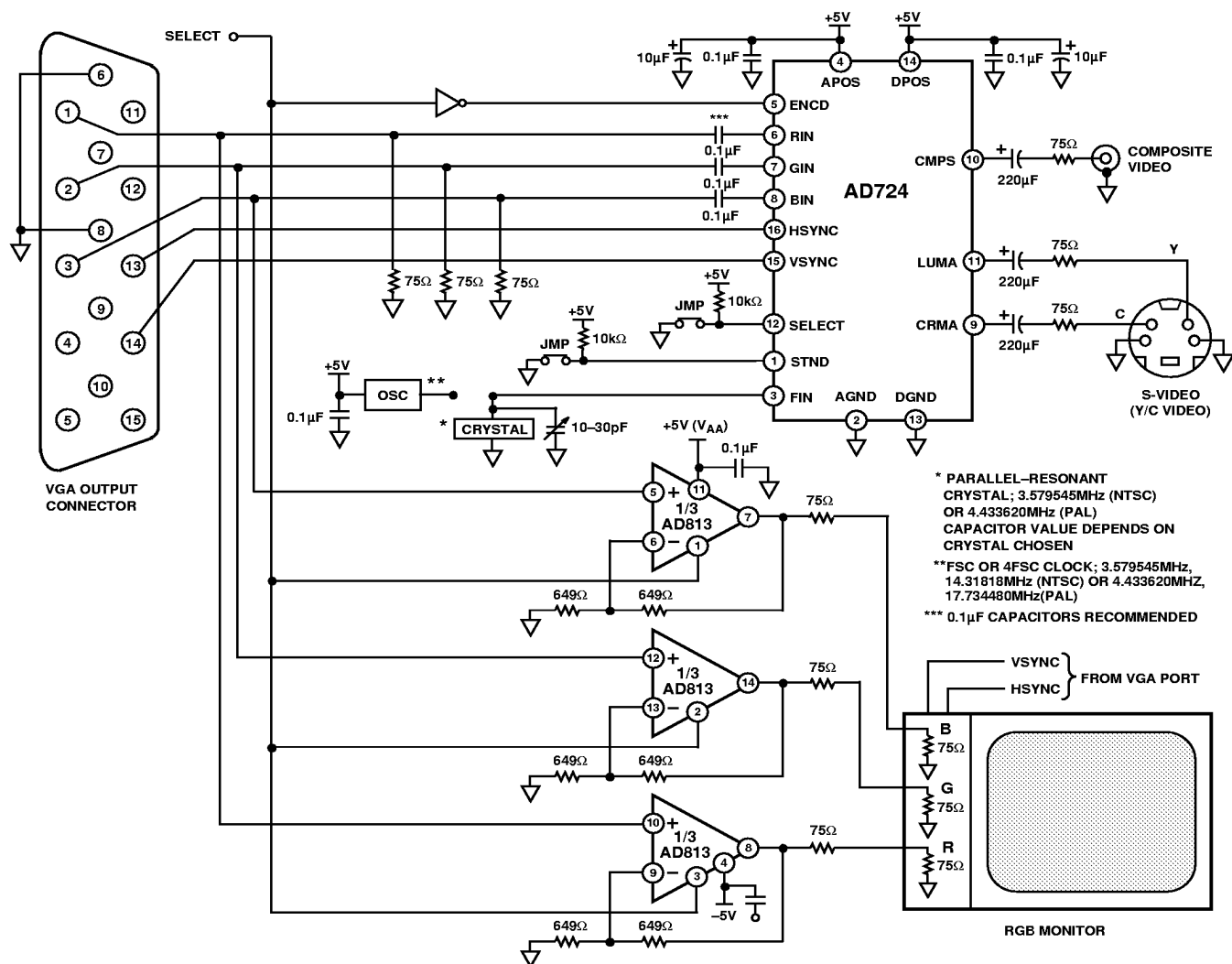
Figure 15. Interfacing the AD724 to the (Interlaced) VGA Port of a PC
