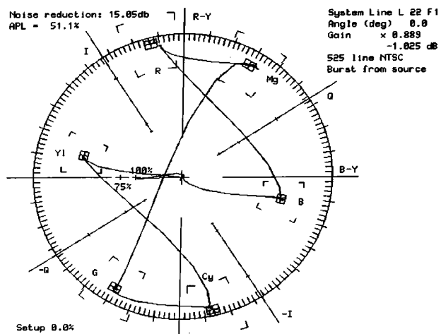
Figure 6. 100% Color Bars on Vector Scope, NTSC
