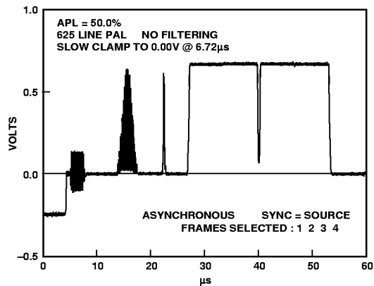
Figure 3. Modulated Pulse and Bar, PAL
