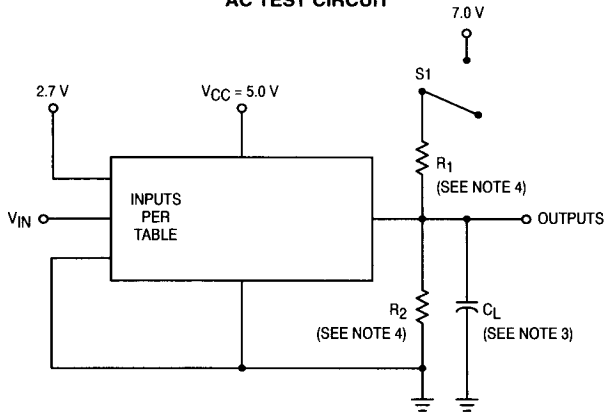
AC TEST CIRCUIT
