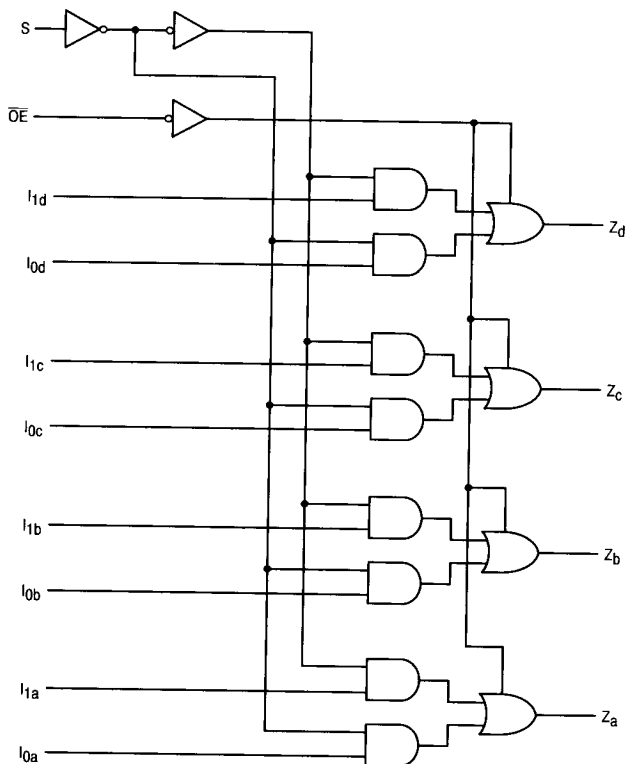
LOGIC DIAGRAM
