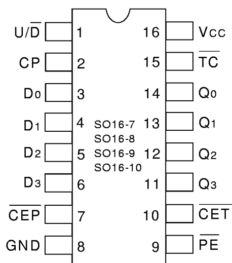
SOIC/ SSOP/ TSSOP/ QSOP TOP VIEW
