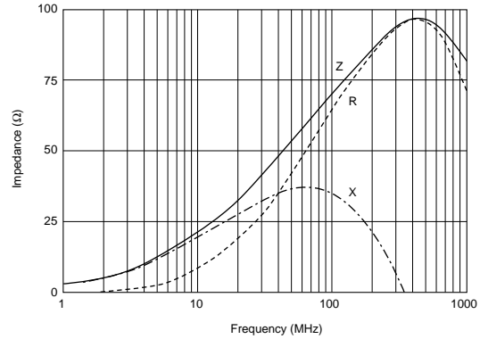
BLM41PG750SN1
