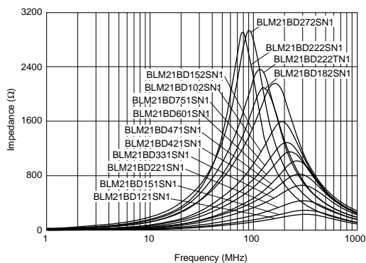
BLM21BD Series
