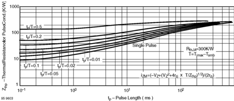
Fig. 10 Thermal Response
