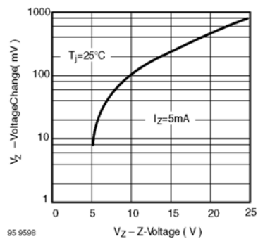
Fig. 2 Typical Change of Working Voltage under Operating Conditions at T amb =25°C
