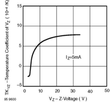
Fig. 4 Temperature Coefficient of Vz vs. Z-Voltage
