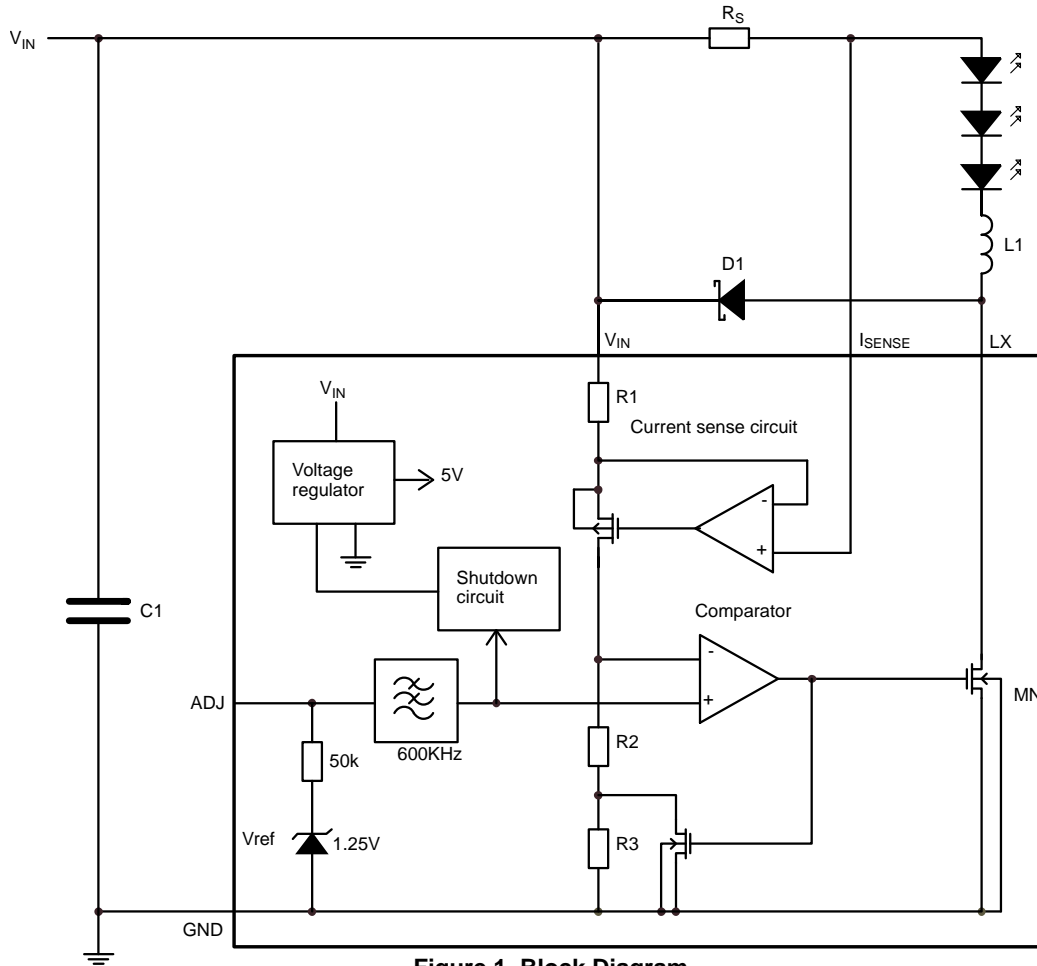
Figure 1. Block Diagram
