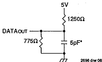
Figure 2. Output Load (for t LZ , t HZ , t WZ , t OW )
