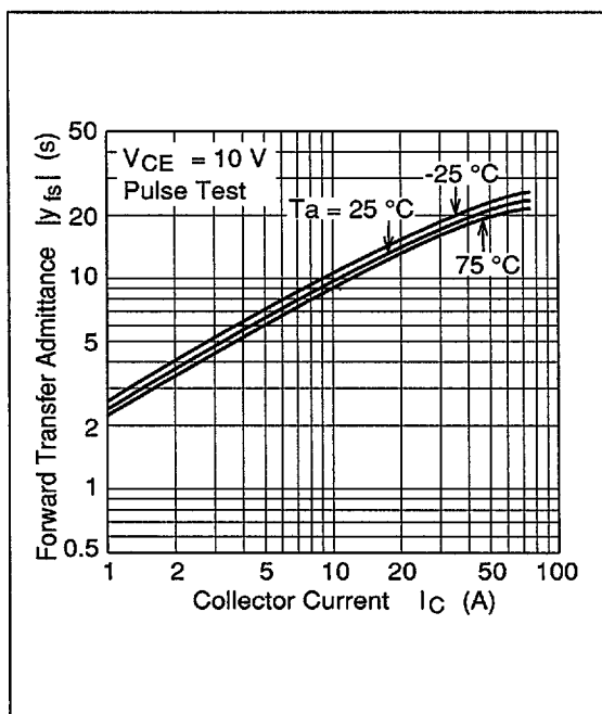
Figure 7 Forward Transfer Admittance vs. Collector Current
