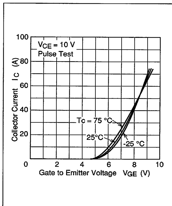
Figure 4 Typical Transfer Characteristics
