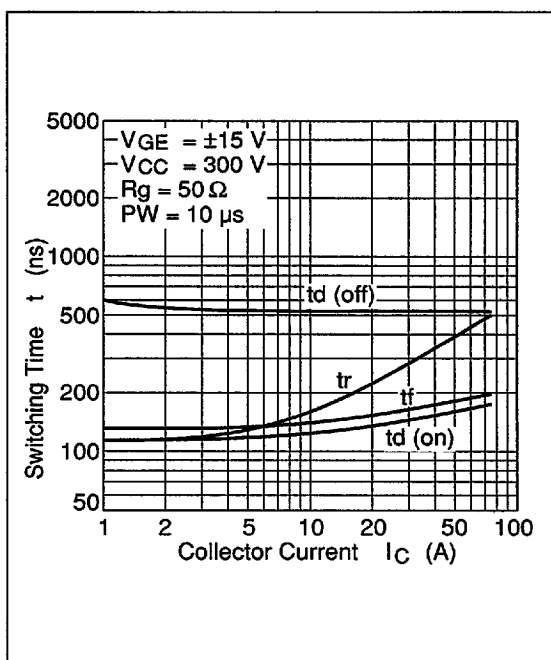
Figure 10 Switching Characteristics
