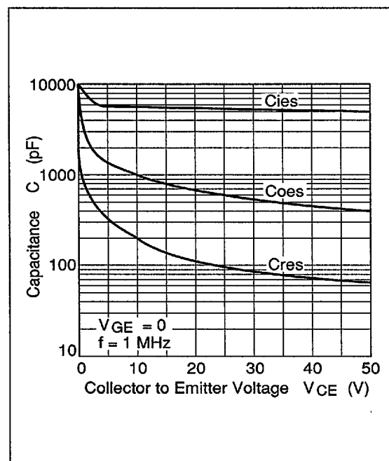
Figure 8 Typical Capacitance vs. Collector to Emitter Voltage
