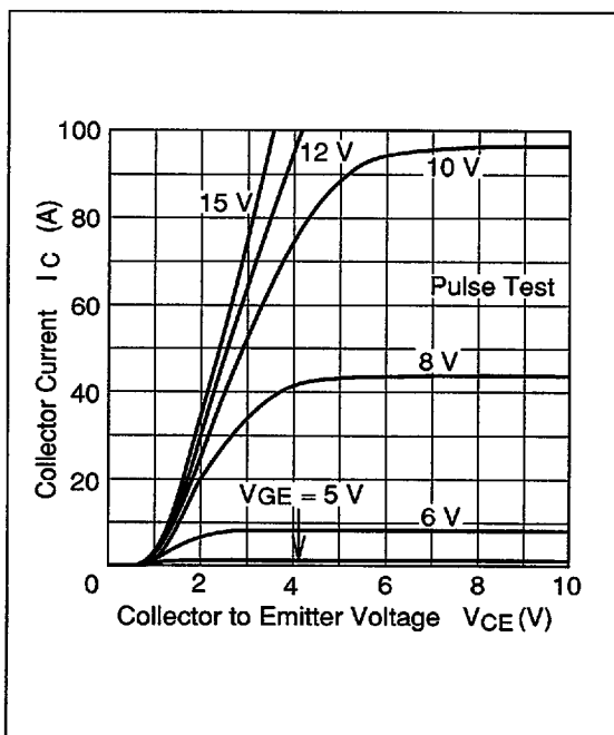
Figure 3 Typical Output Characteristics
