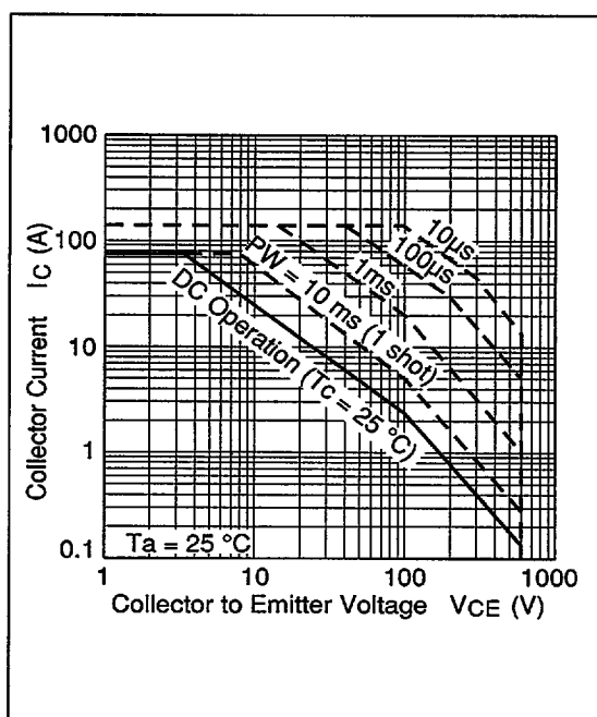
Figure 2 Maximum Safe Operation Area
