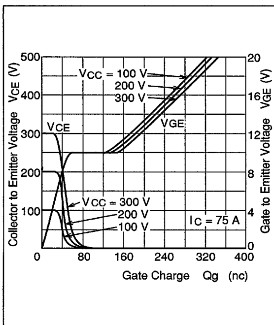
Figure 9 Dynamic Input Characteristics
