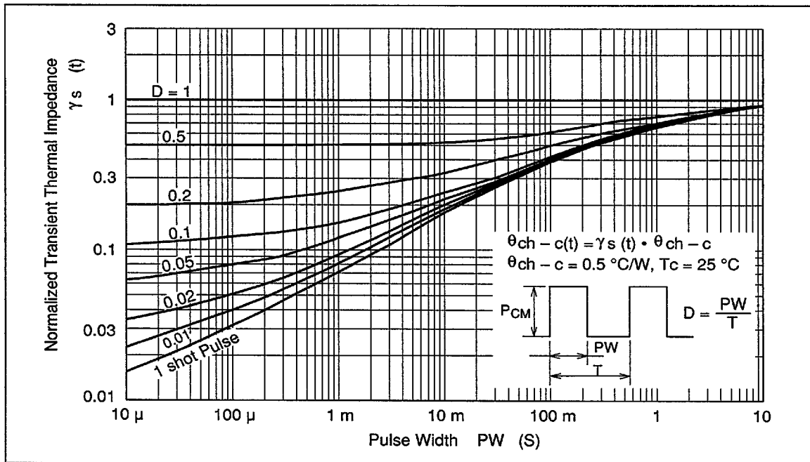
Figure 12 Normalized Transient Thermal Impedance vs. Pulse Width
