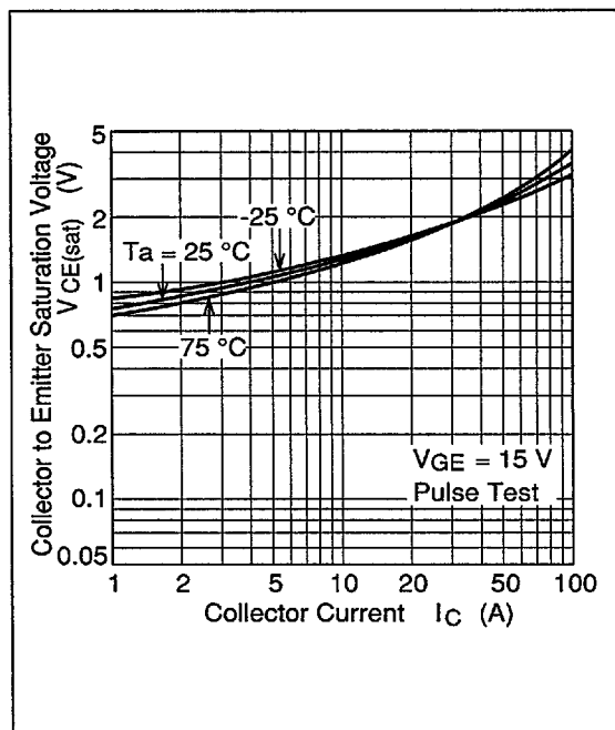
Figure 6 Collector to Emitter Saturation Voltage vs. Collector Current
