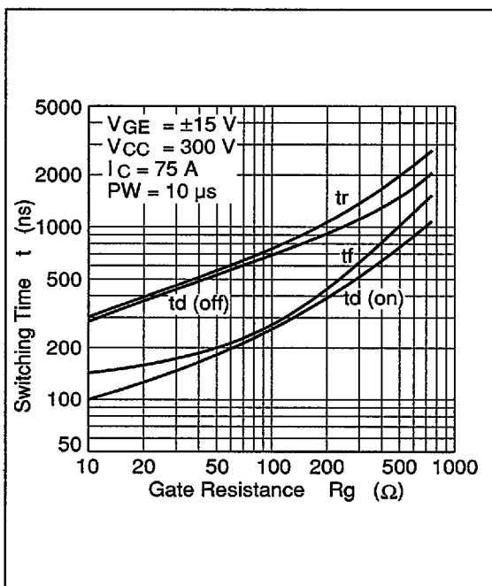
Figure 11 Switching Characteristics
