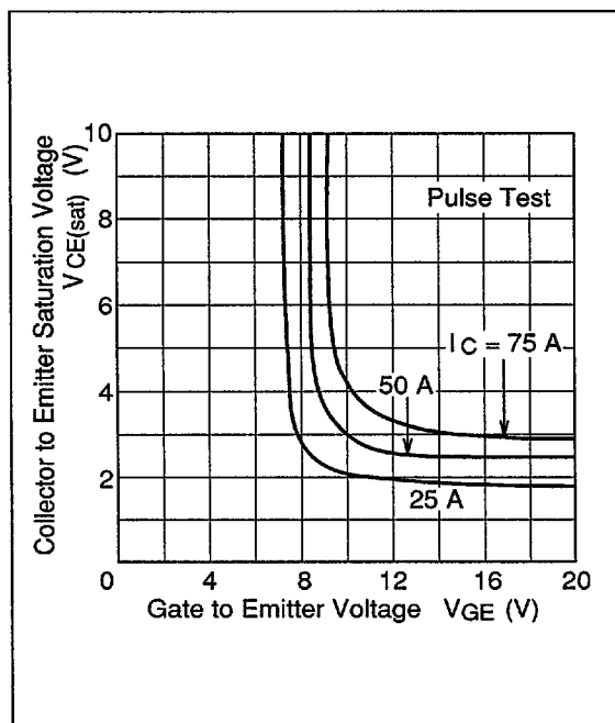
Figure 5 Collector to Emitter Saturation Voltage vs. Gate to Emitter Voltage
