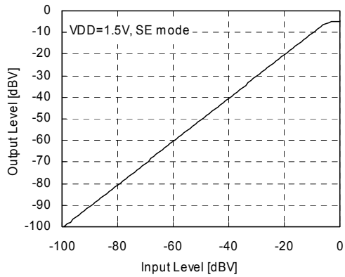
Fig. 10 Output Level vs. Input Level
