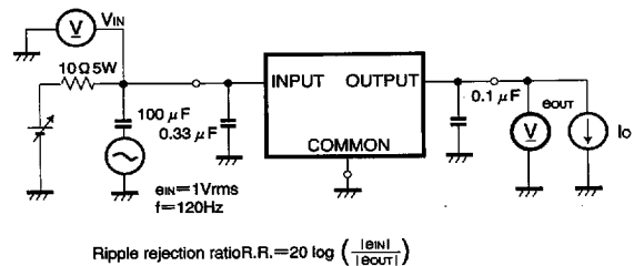
Fig. 6 Measurement circuit for ripple rejection
