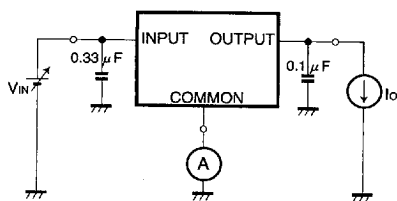
Fig. 9 Measurement circuit for bias current and bias current change
