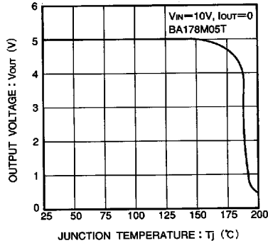
Fig. 2 Thermal cutoff circuit characteristic
