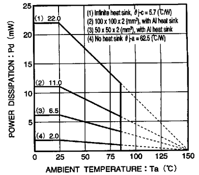
Fig. 3 Ta - power consumption characteristic (TO220FP)
