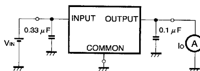
Fig. 10 Measurement circuit for short-circuit output current
