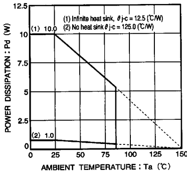
Fig. 4 Ta - power consumption characteristic (TO252-3)
