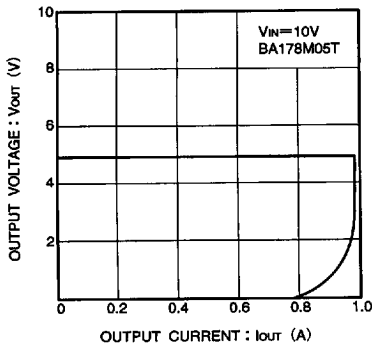
Fig. 1 Current limit characteristic
