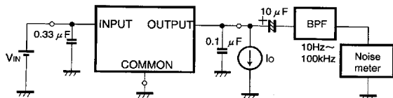
Fig. 7 Measurement circuit for output noise voltage
