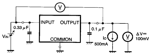
Fig. 8 Measurement circuit for dropout voltage
