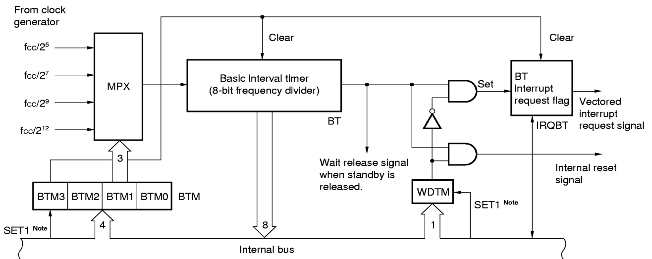
Figure 6-3. Basic Interval Timer/Watchdog Timer Block Diagram
