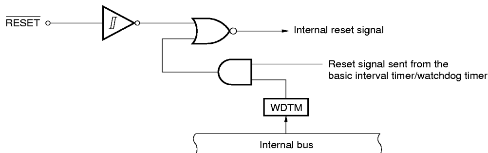
Figure 9-1. Configuration of Reset Function
