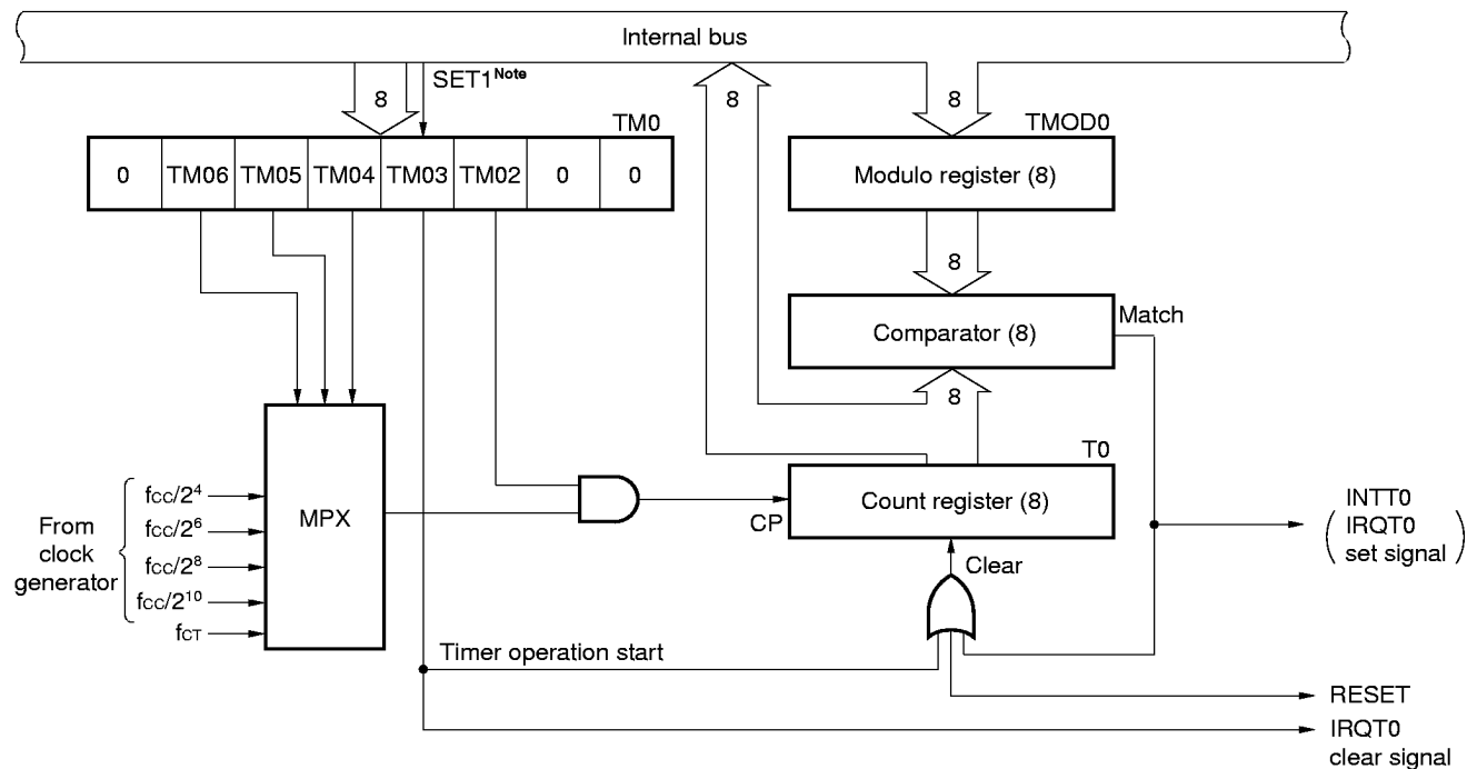
Figure 6-5. Timer Counter Block Diagram
