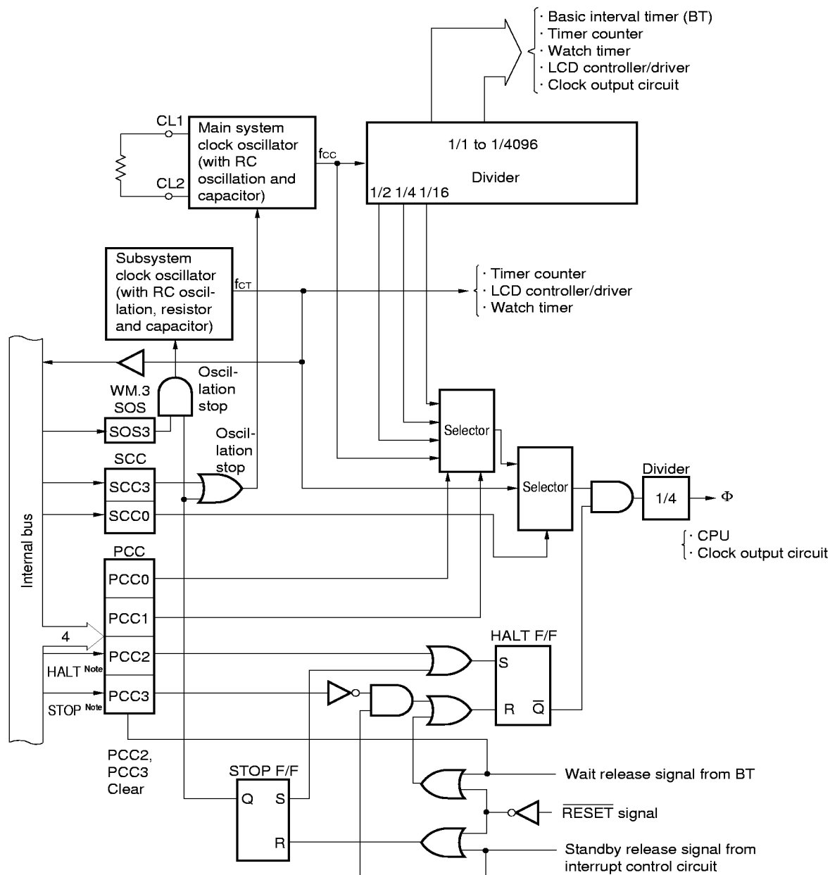
Figure 6-1. Clock Generator Block Diagram
