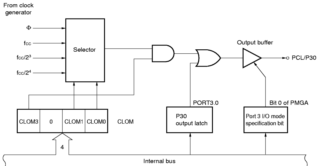
Figure 6-2. Clock Output Circuit Block Diagram
