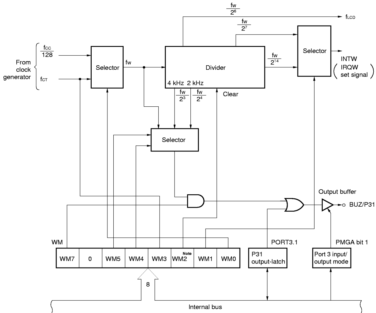
Figure 6-4. Watch Timer Block Diagram
