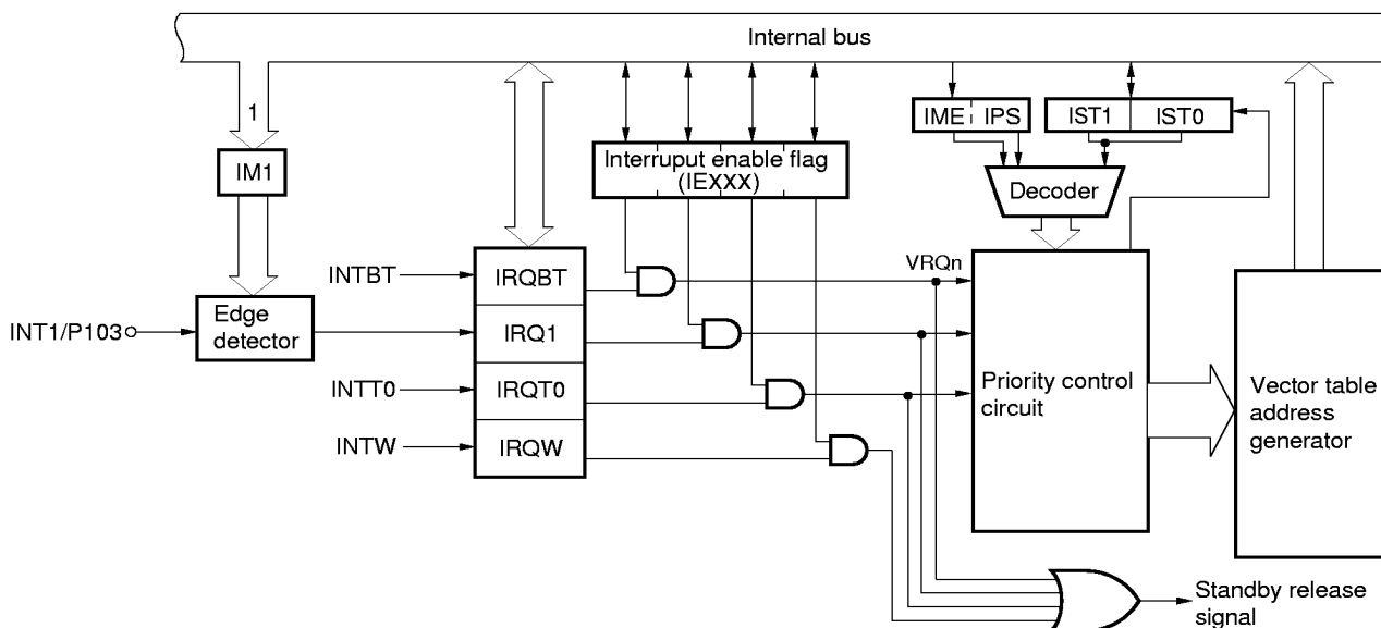
Figure 7-1. Interrupt Control Circuit Block Diagram
