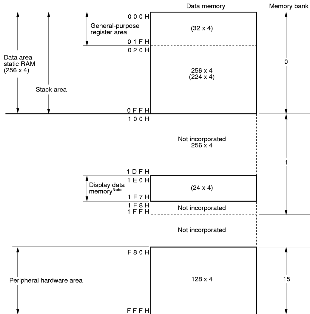
Figure 5-2. Data Memory Map
