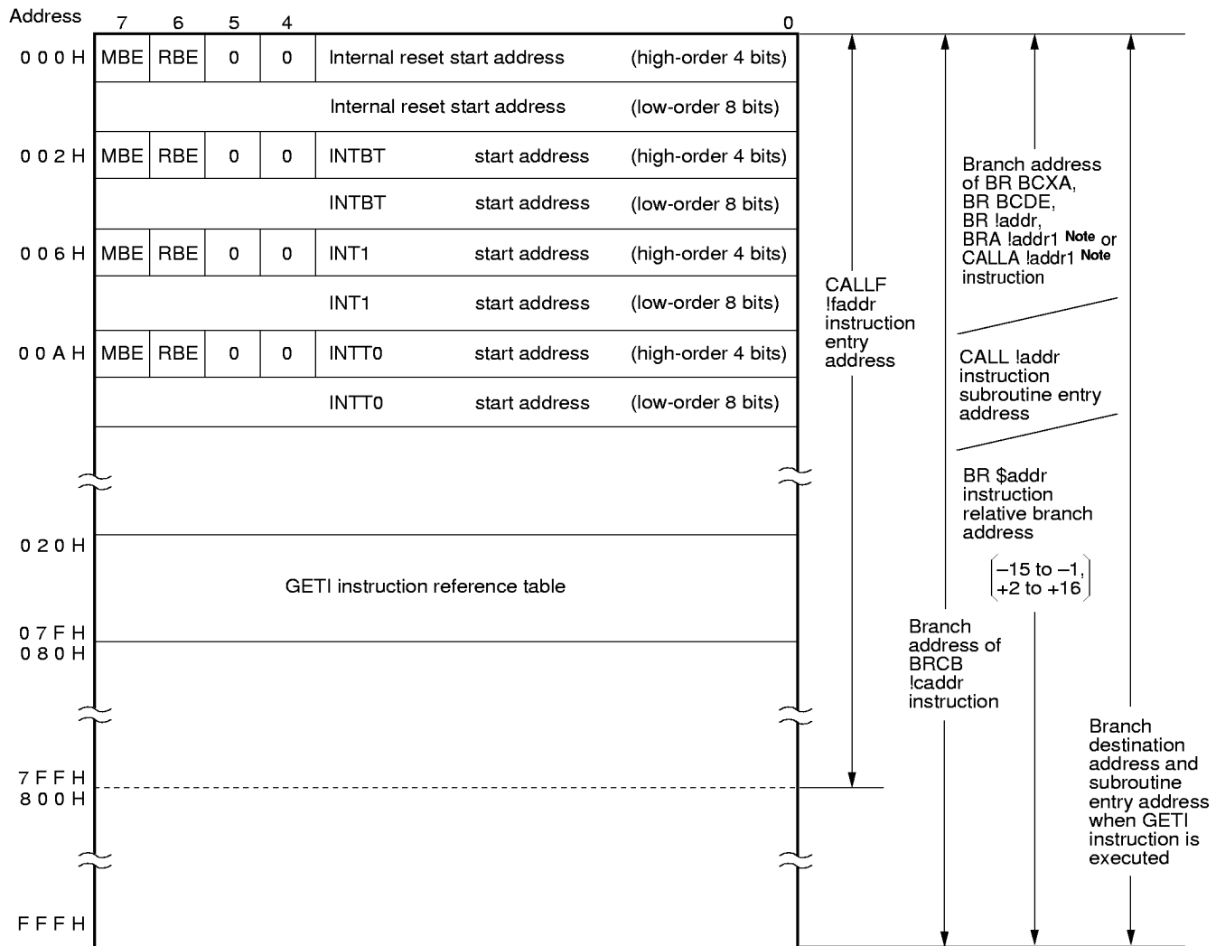
Figure 5-1. Program Memory Map
