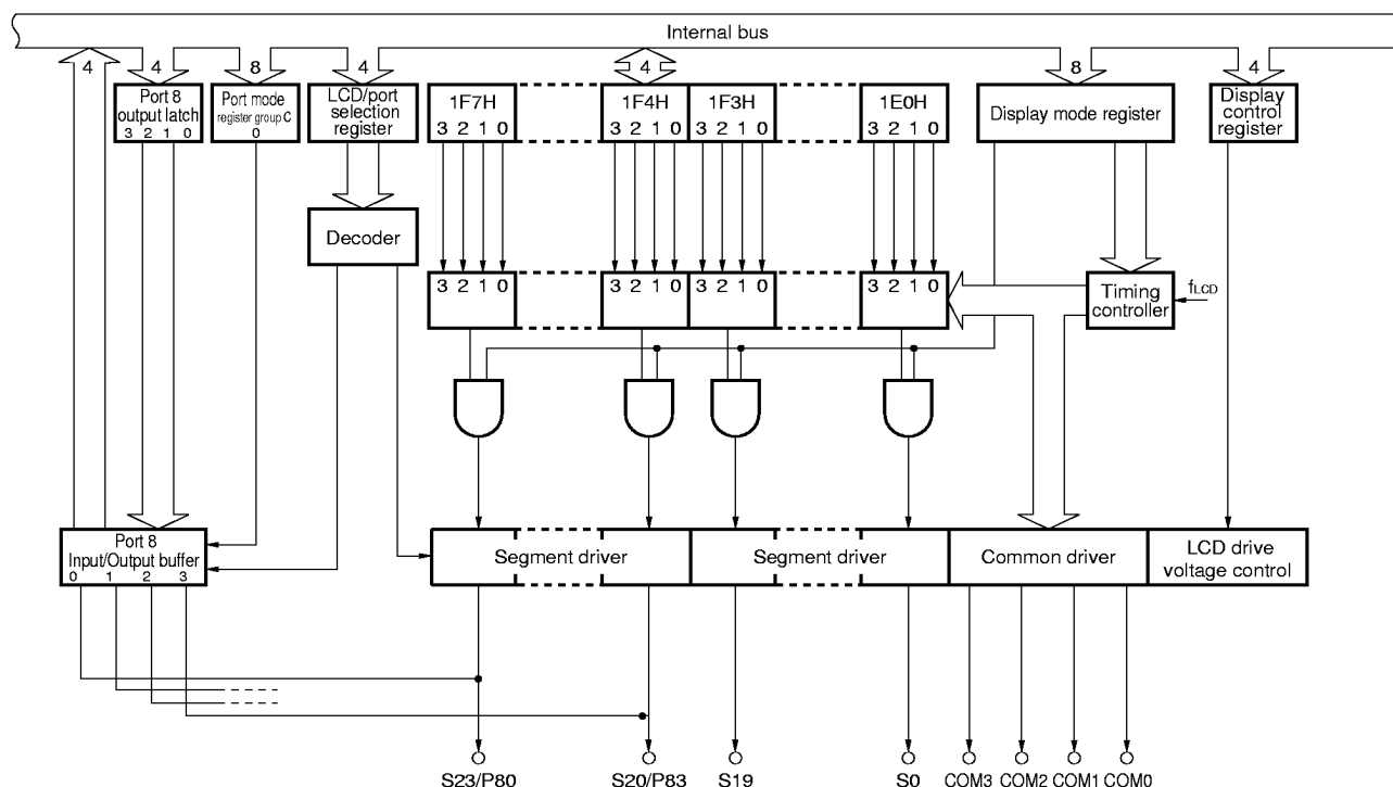
Figure 6-6. LCD Controller/Driver Block Diagram
