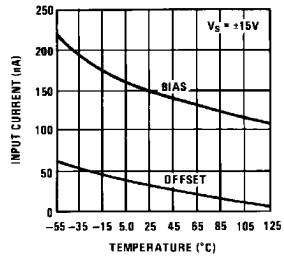
Input Currents
