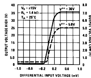
Transfer Function
