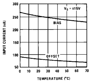
Input Currents
