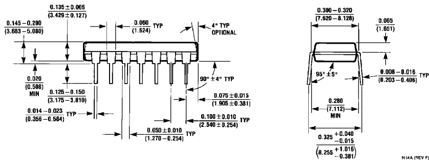
Molded Dual-In-Line Package (N) Order Number LM319AN or LM319N NS Package Number N14A
