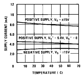
Supply Currents
