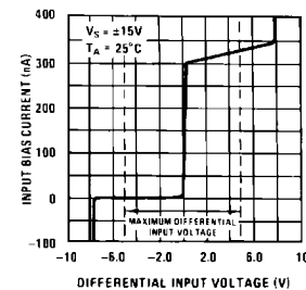
Input Characteristics
