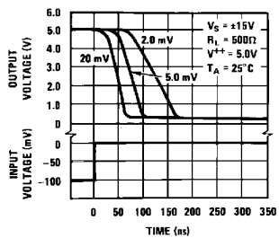
Response Time for Various Input Overdrives
