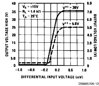
Input Characteristics
