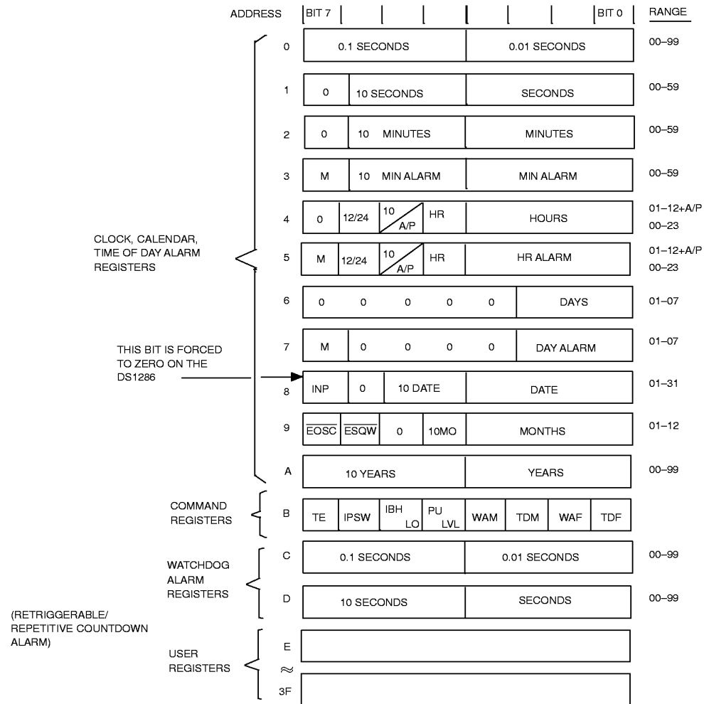
DS1283 WATCHDOG TIMEKEEPER REGISTERS Figure 1
