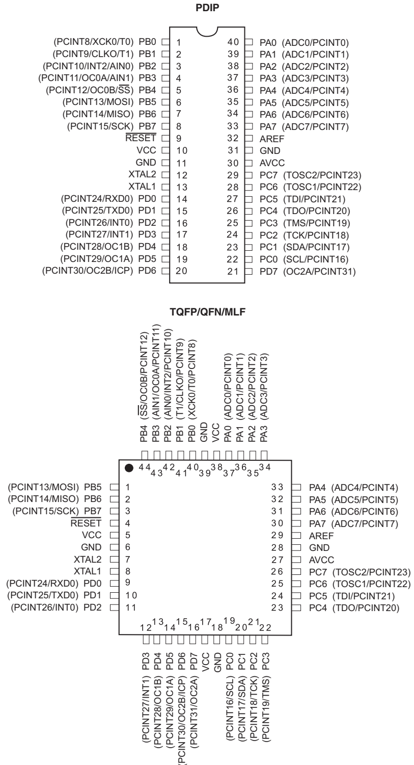
Figure 2. Pinout ATmega644
