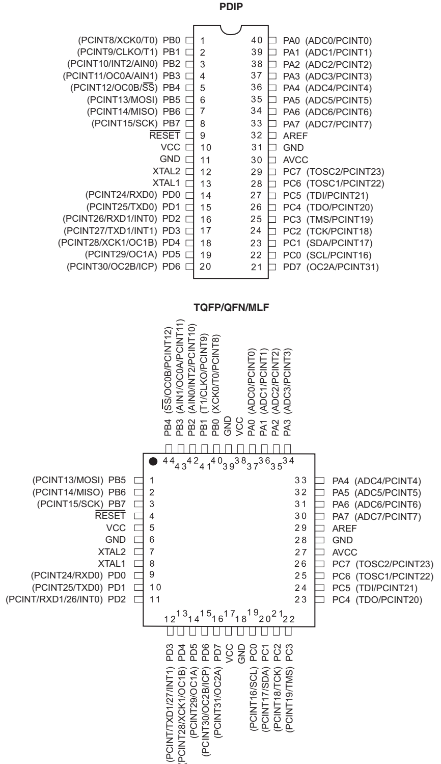
Figure 1. Pinout ATmega164/324
