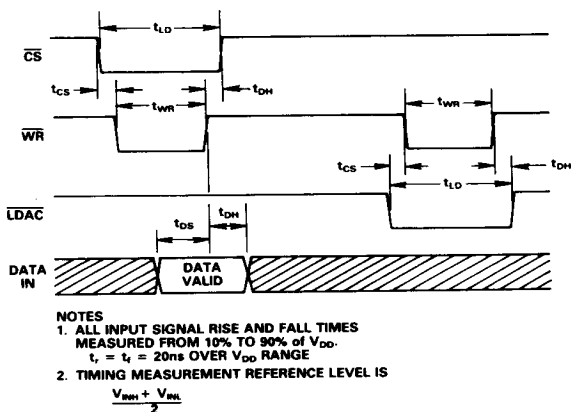
Figure 2. Write Cycle Timing Diagram
