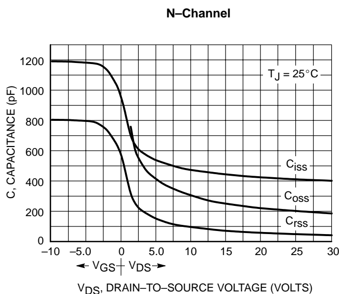
Figure 7. Capacitance Variation
