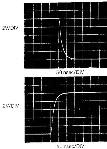
DAC-HF with AM-500, \pm 5V output full scale (10V) step
