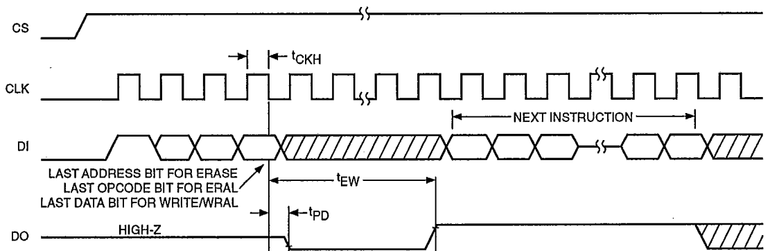
Figure 5. Program/Erase Timing
