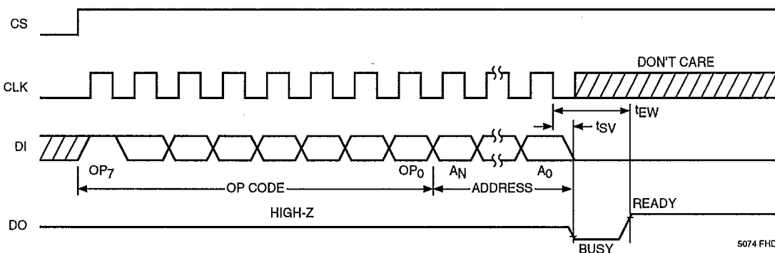
Figure 10. Erase Timing
