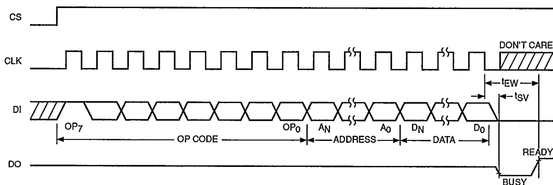
Figure 8. Write Timing
