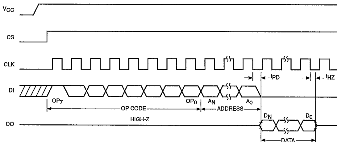
Figure 7. Read Timing
