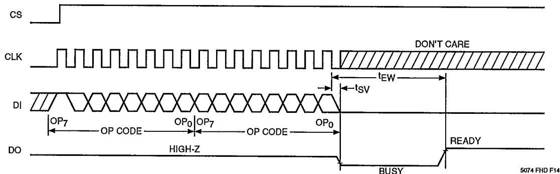
Figure 11. ERAL Timing
