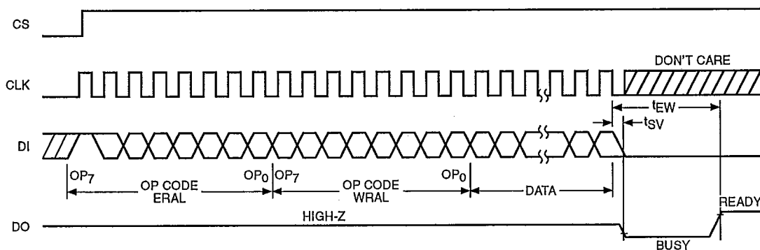
Figure 12. WRAL Timing
