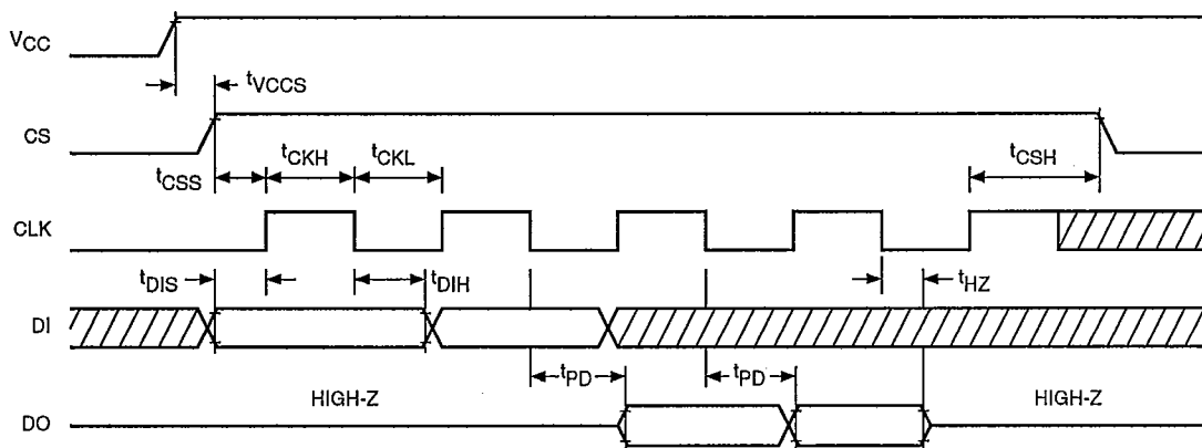
Figure 1. A.C. Timing
