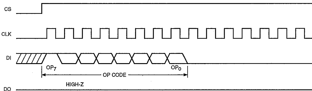
Figure 9. EWEN/EWDS Timing
