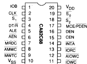
Figure 2 : PLCC and DIP PIN CONFIGURATIONS
