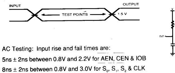
Figure 4 : AC TESTING I/O WAVEFORM
