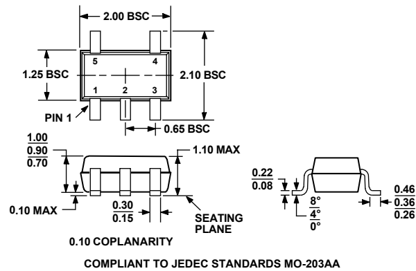
Figure 15. 5-Lead Plastic Surface-Mount Package [SC-70] (KS-5) Dimensions shown in millimeters
