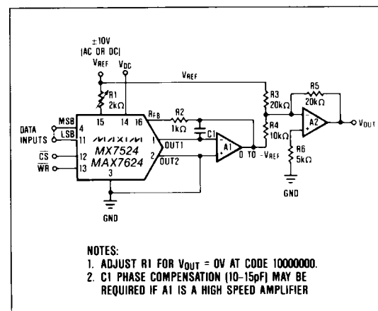
Figure 4. Bipolar (4-Quadrant) Operation
