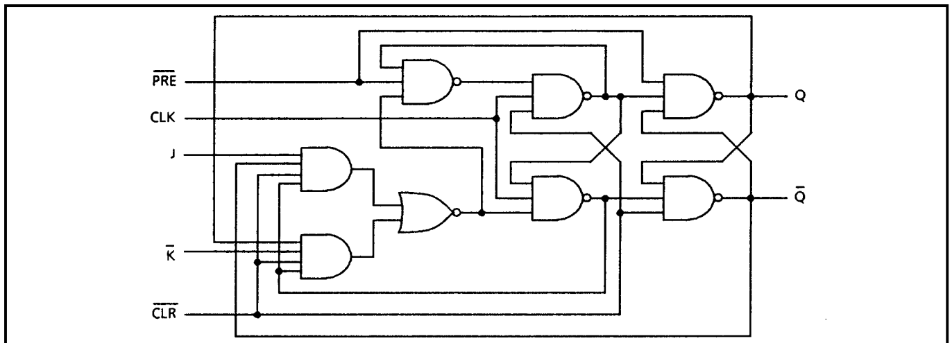
Figure 3: Logic Diagram
