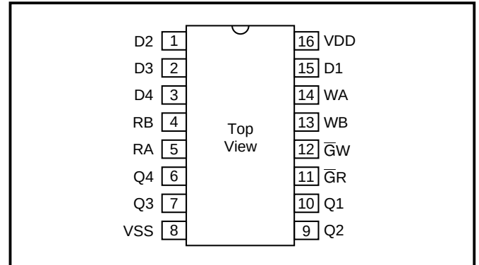
Figure 1: Pin Out
