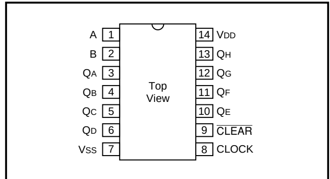
Figure 2: Pin Out
