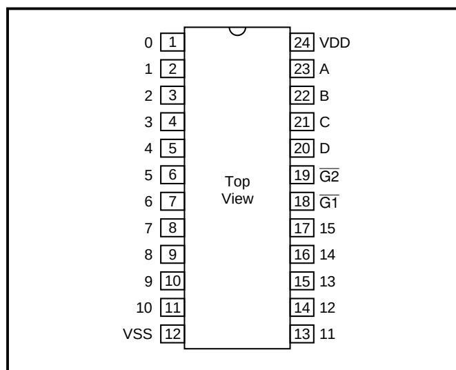
Figure 2: Pin Out
