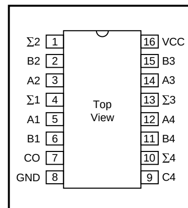
Figure 2: Pin Out
