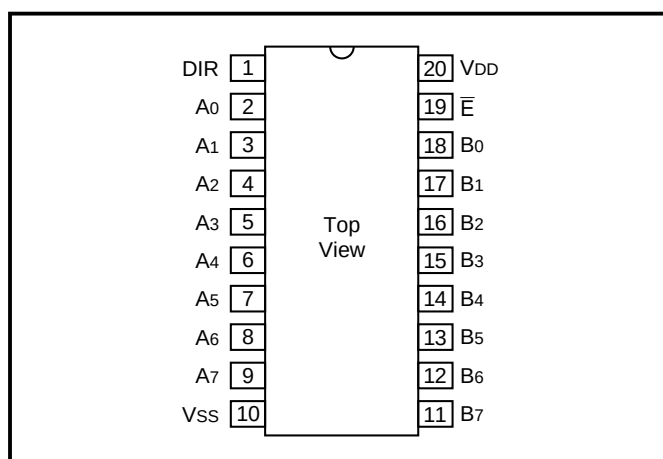
Figure 2: Pin Out
