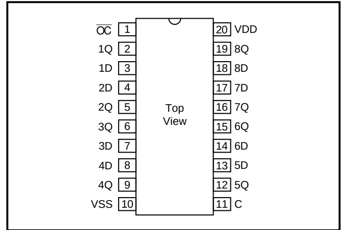
Figure 2: Pin Out
