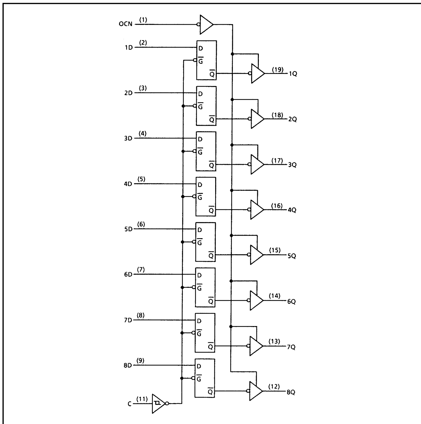
Figure 5: Logic Diagram
