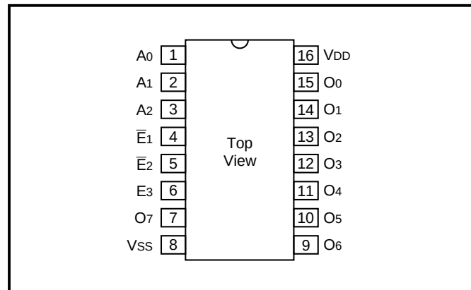
Figure 2: Pin Out
