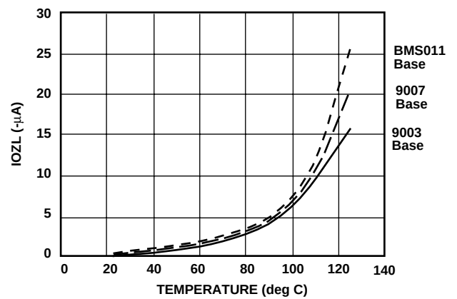
IOZL Vs TEMP.
