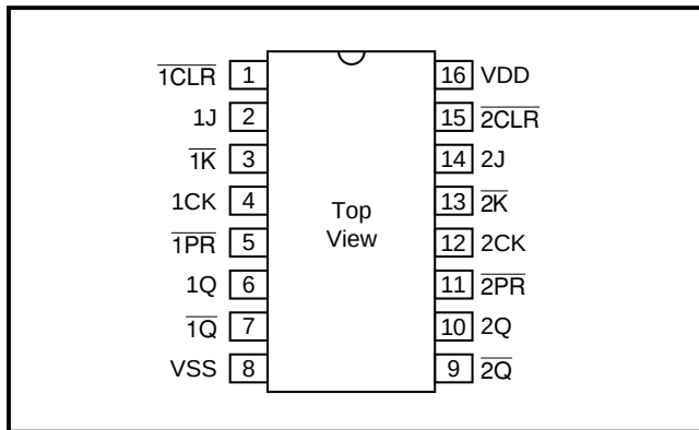
Figure 1: Pin Out
