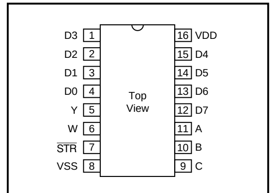
Figure 2: Pin Out
