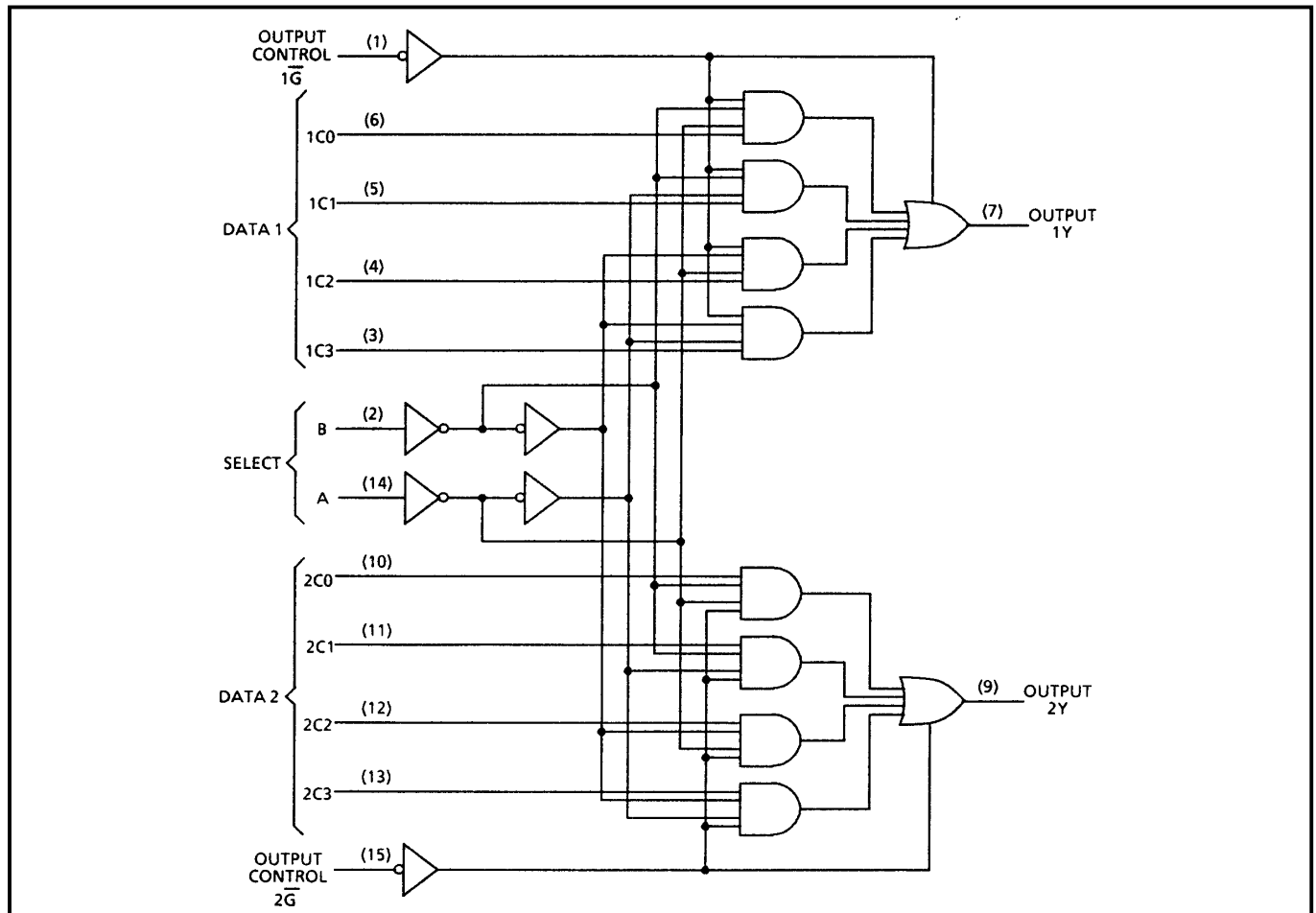
Figure 5: Logic Diagram
