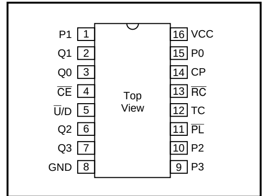
Figure 2: Pin Out
