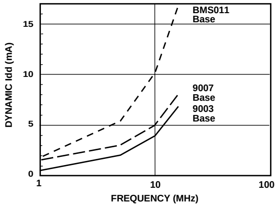
DYNAMIC I dd for OCTAL DEVICE BASES
