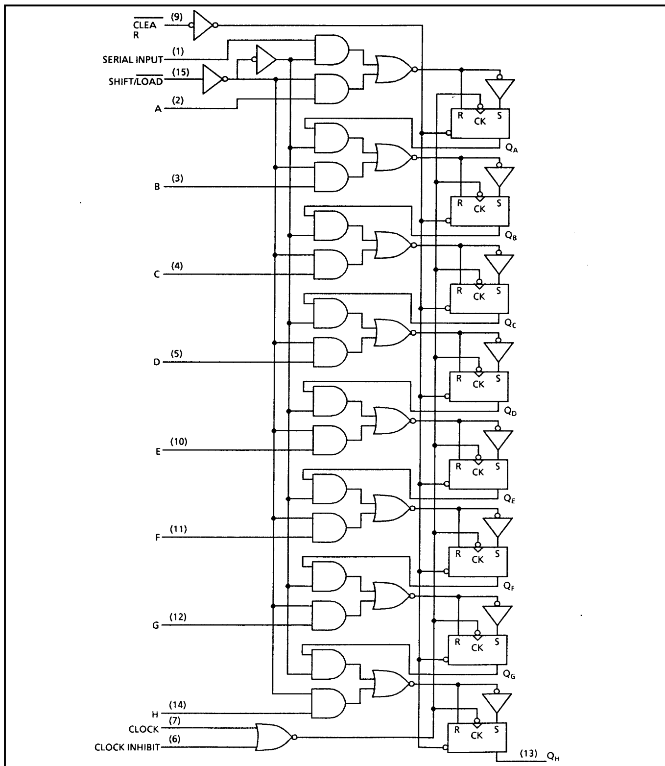
Figure 5: Logic Diagram
