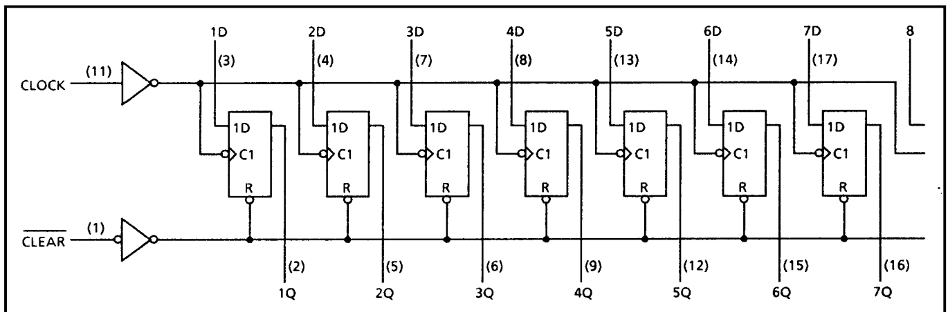
Figure 3: Logic Diagram
