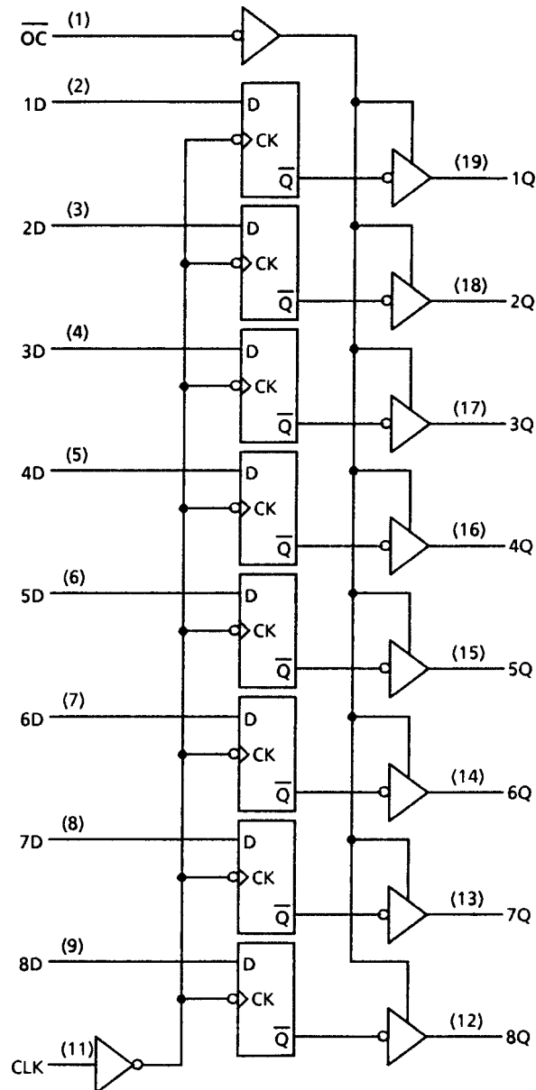
Figure 5: Logic Diagram
