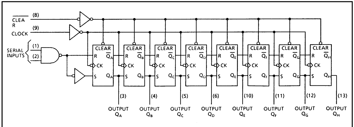
Figure 5: Logic Diagram
