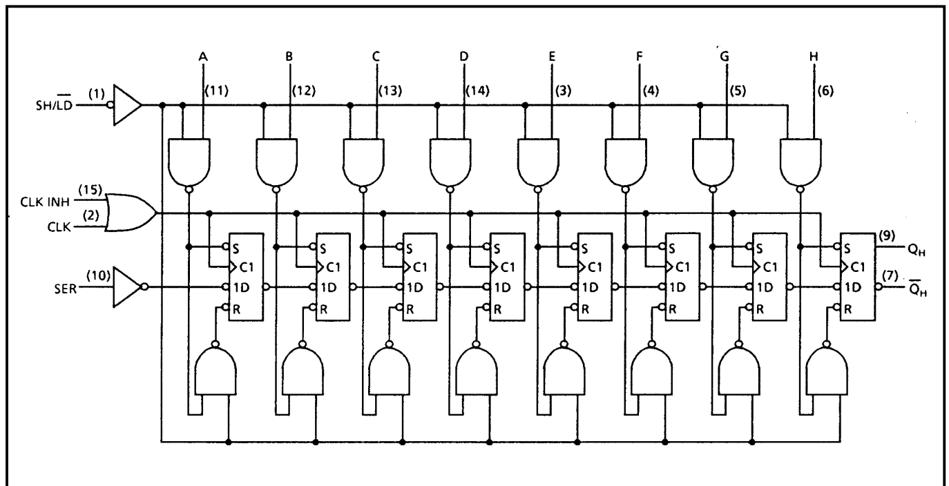
Figure 5: Logic Diagram
