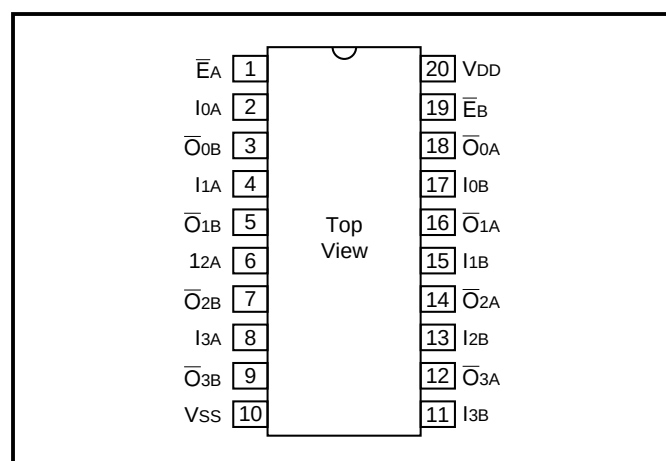
Figure 2: Pin Out
