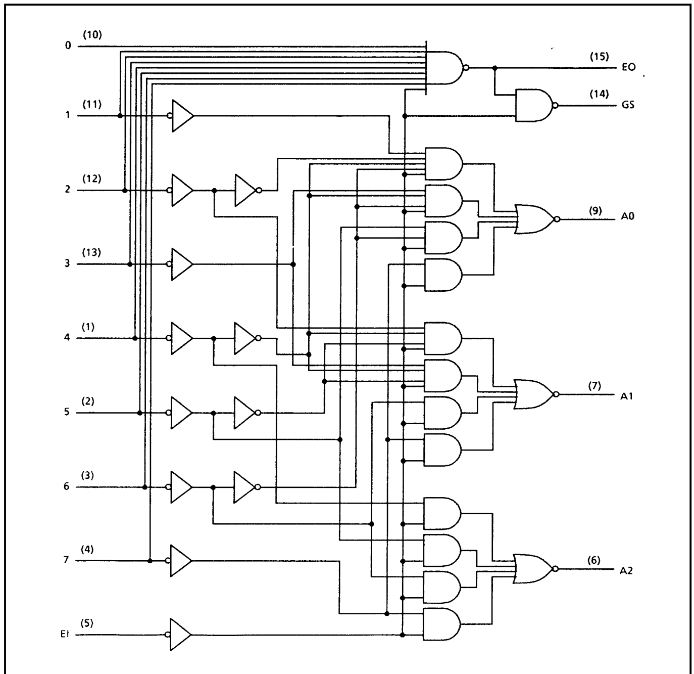
Figure 5: Logic Diagram
