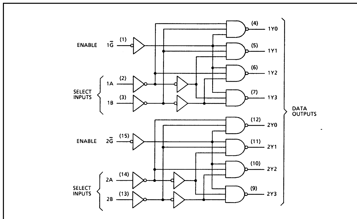
Figure 5: Logic Diagram
