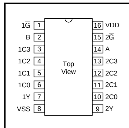
Figure 2: Pin Out
