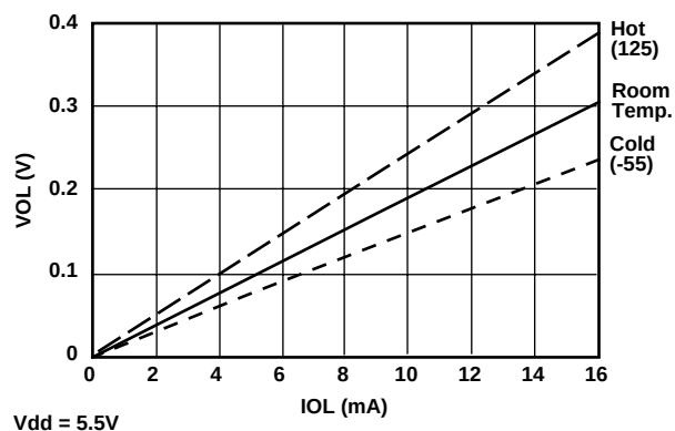
VOL Vs IOL BMS011 Base
