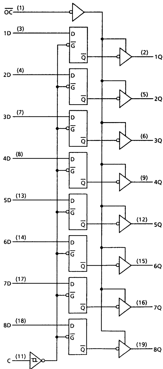
Figure 5: Logic Diagram
