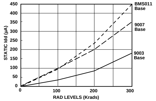
STATIC I dd Vs RADIATION
