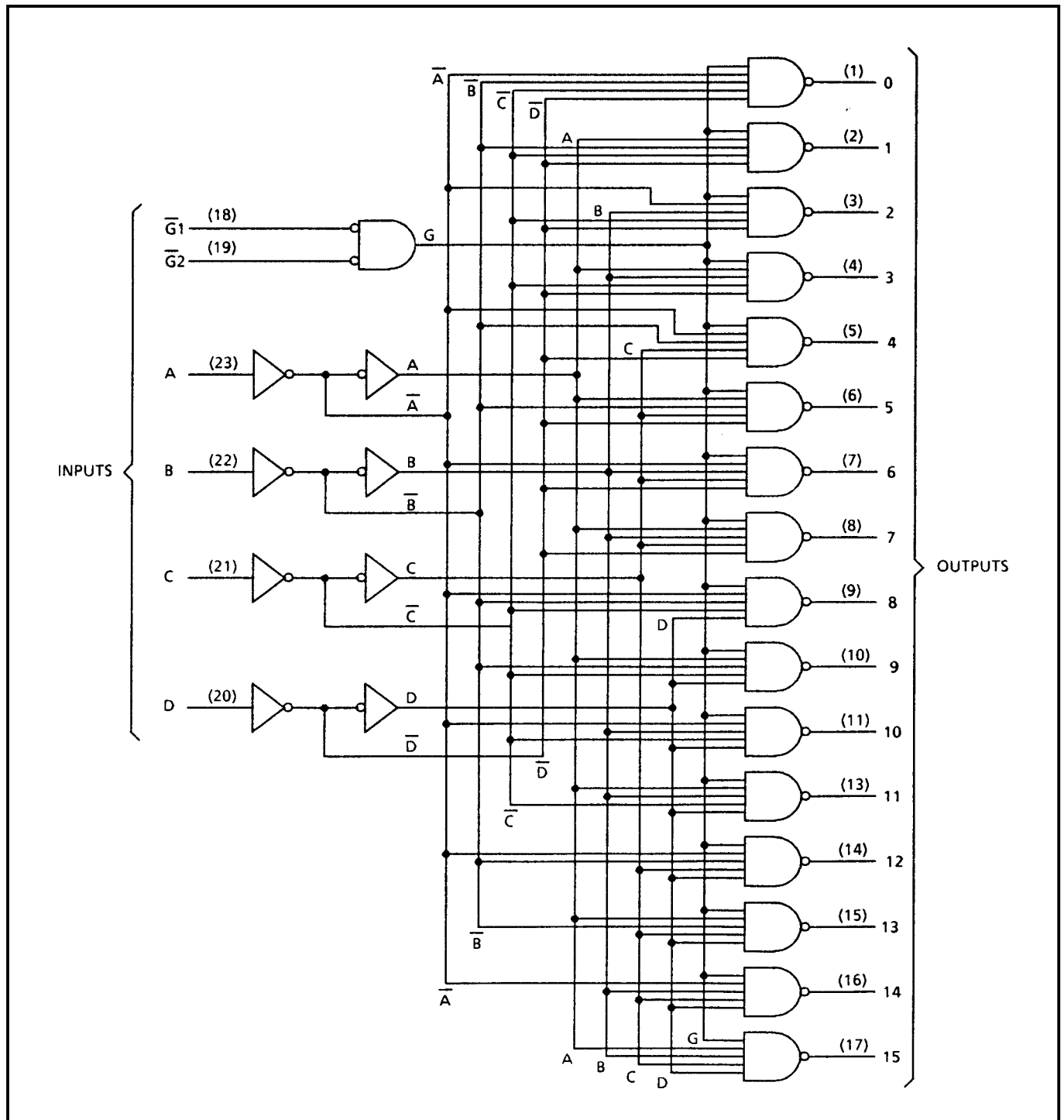
Figure 5: Logic Diagram
