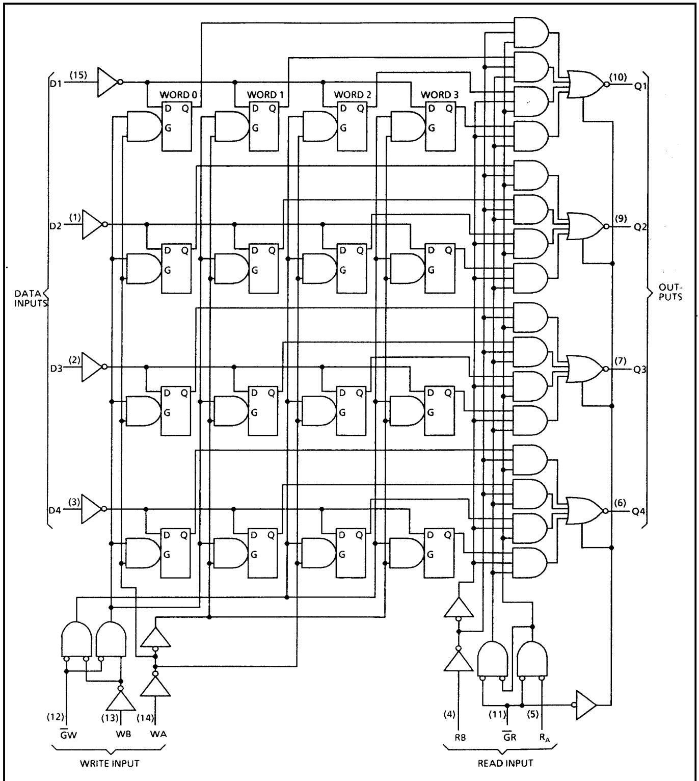
Figure 6: Logic Diagram
