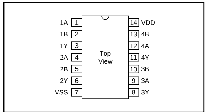
Figure 3: Pin Out
