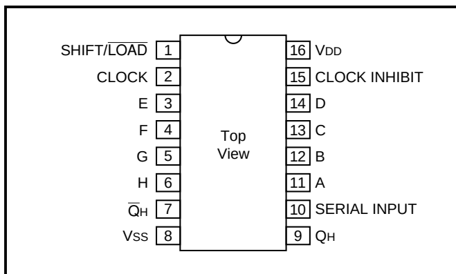
Figure 2: Pin Out
