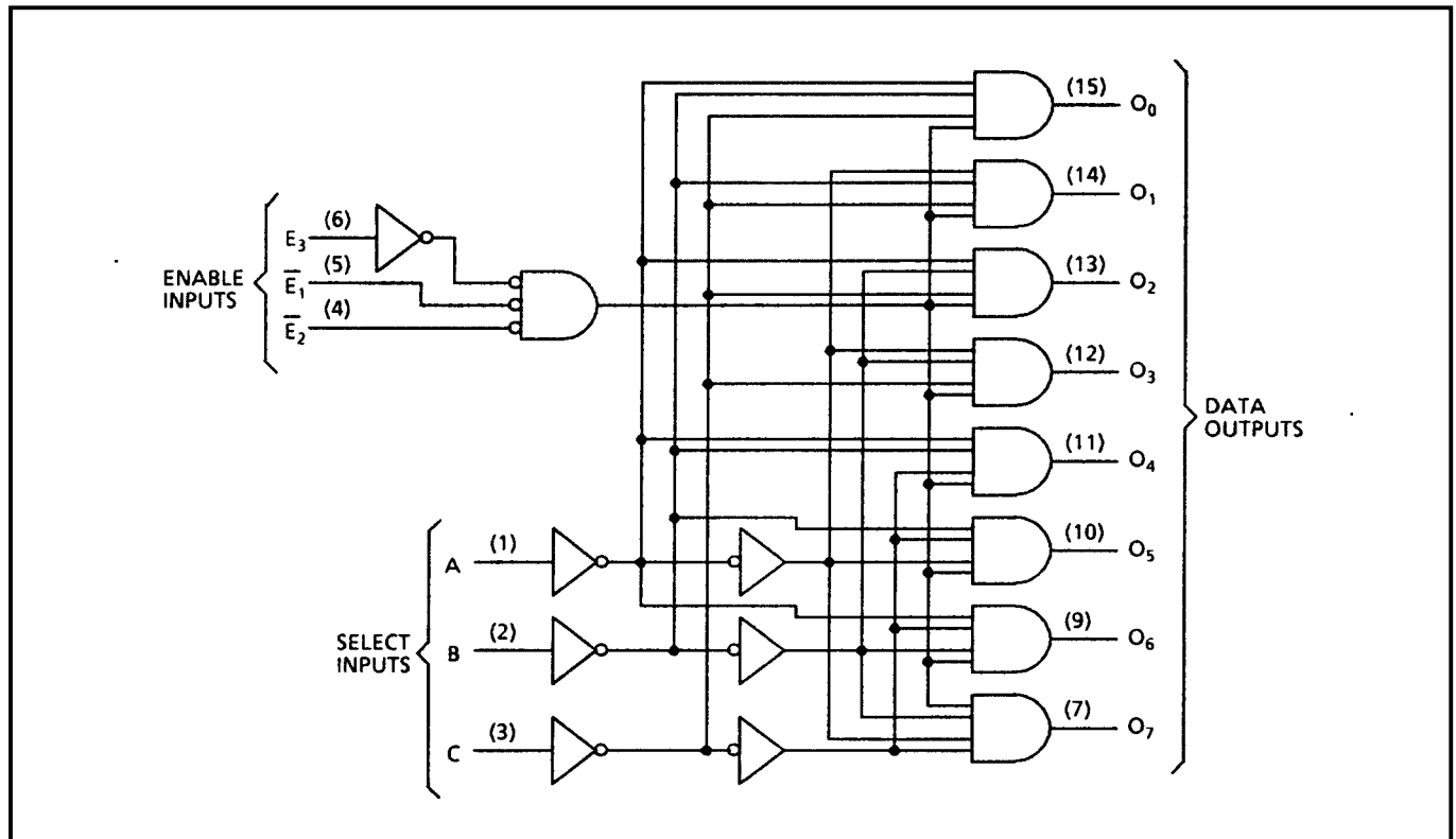
Figure 5: Logic Diagram
