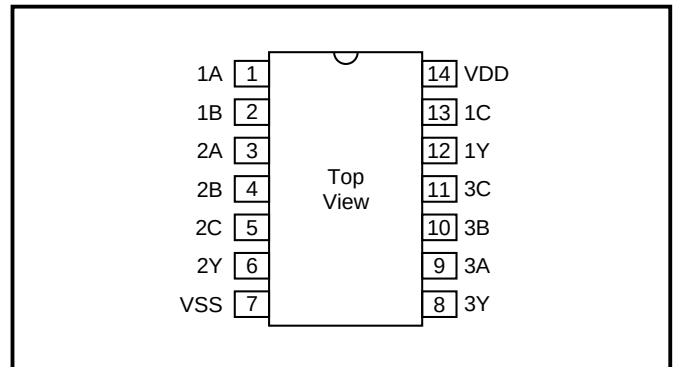
Figure 3: Pin Out
