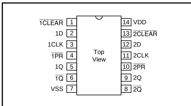
Figure 3: Pin Out
