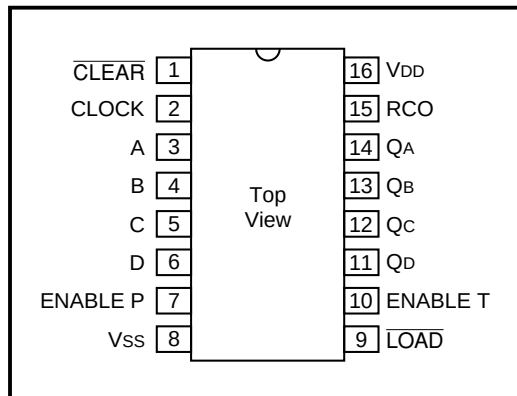
Figure 2: Pin Out
