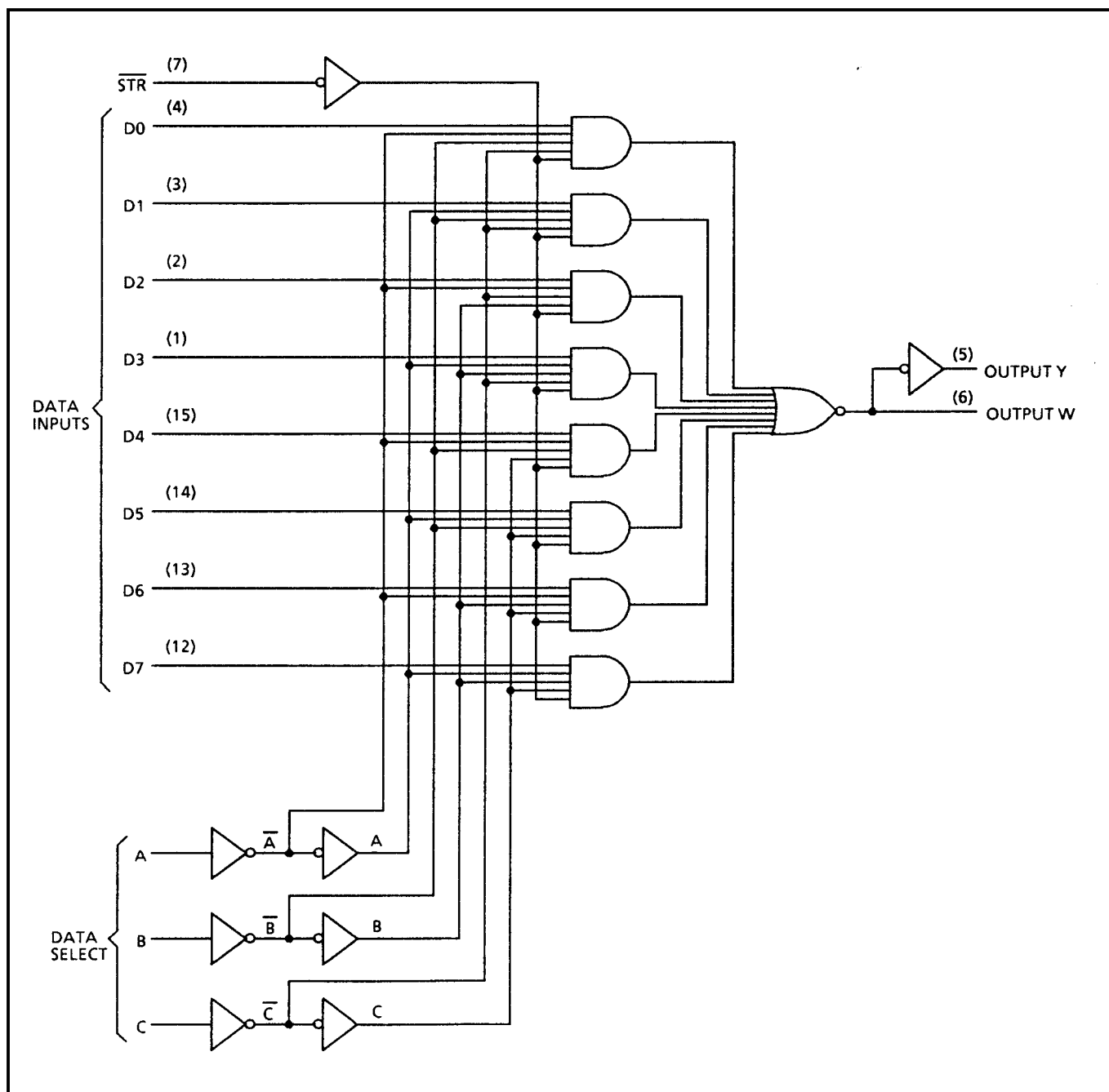
Figure 5: Logic Diagram
