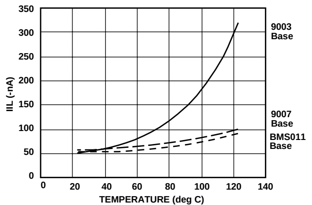
IIL Vs TEMP.
