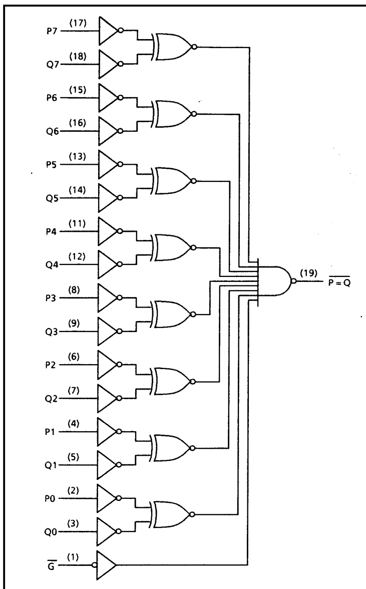
Figure 3: Logic Diagram
