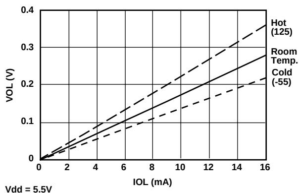
VOL Vs IOL MA9007 Base
