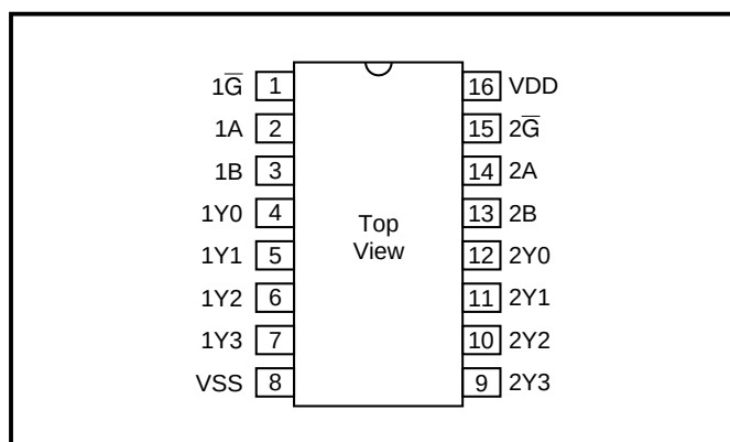
Figure 2: Pin Out
