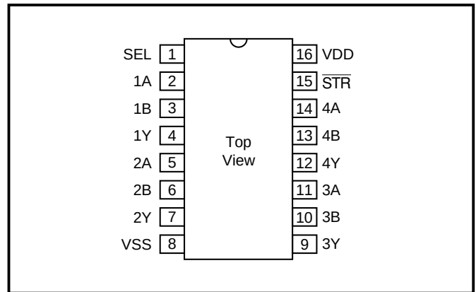
Figure 2: Pin Out
