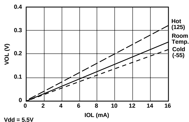
VOL Vs IOL MA9003 Base
