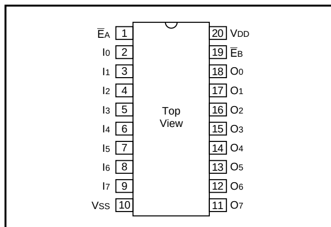
Figure 2: Pin Out
