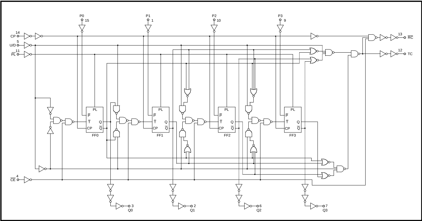
Figure 5: Logic Diagram
