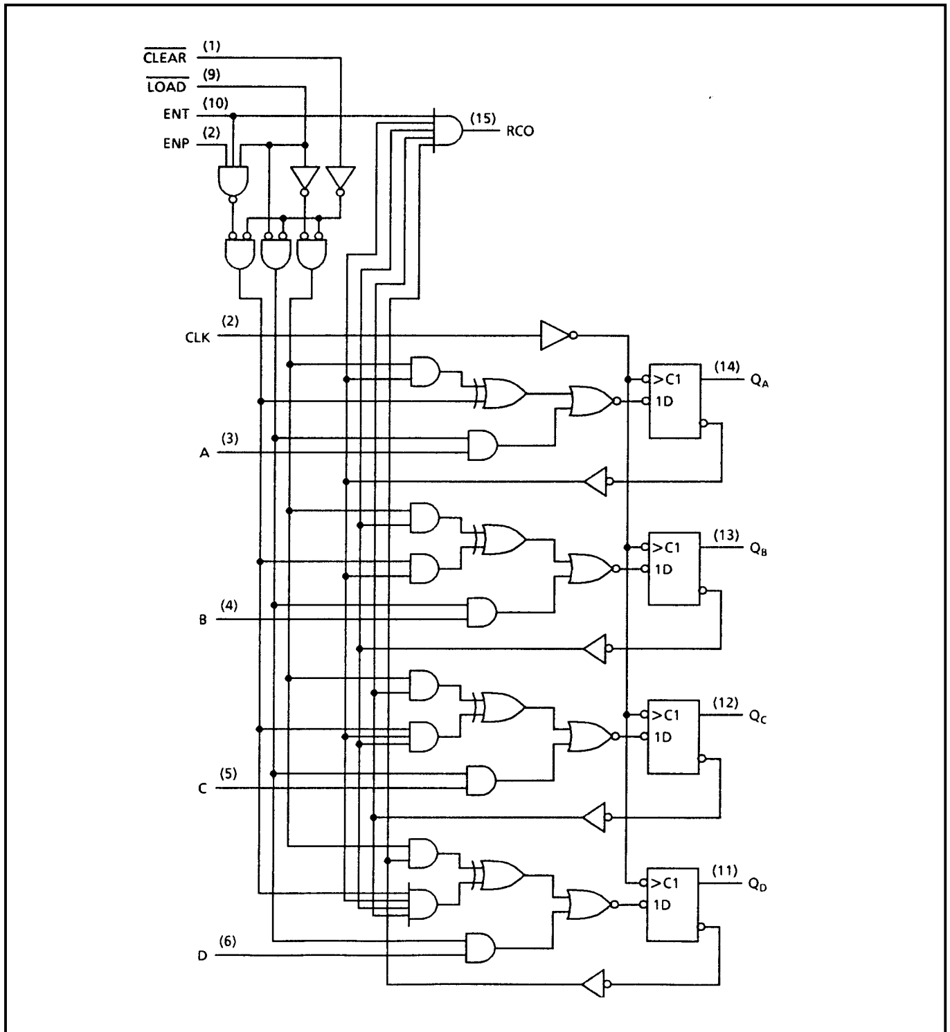
Figure 5: Logic Diagram
