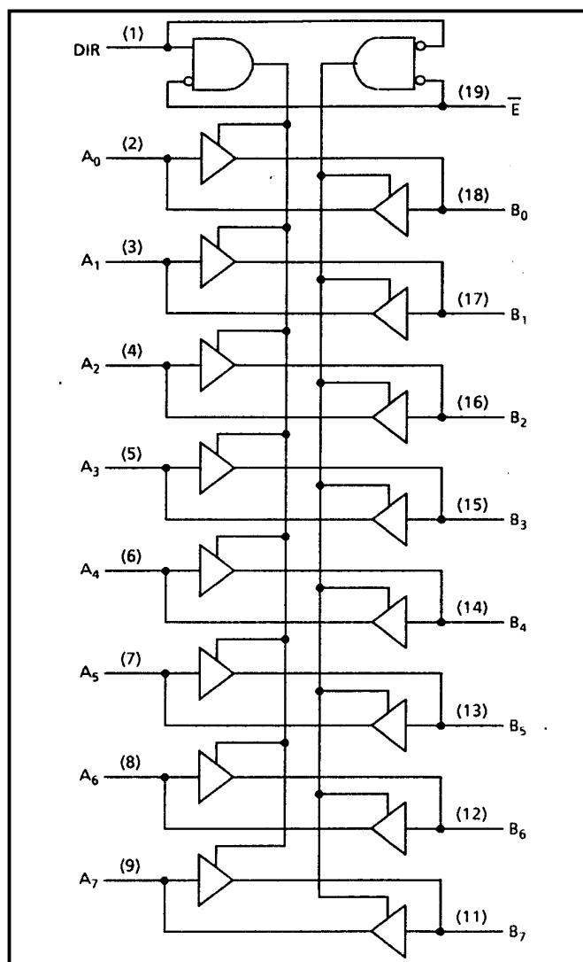
Figure 3: Logic Diagram
