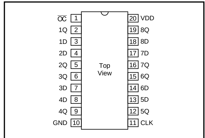
Figure 2: Pin Out
