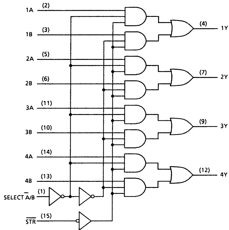
Figure 5: Logic Diagram
