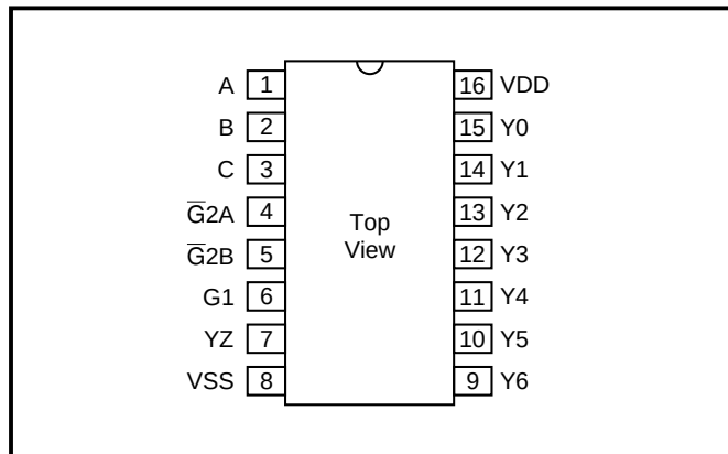
Figure 2: Pin Out
