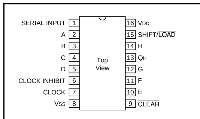
Figure 2: Pin Out
