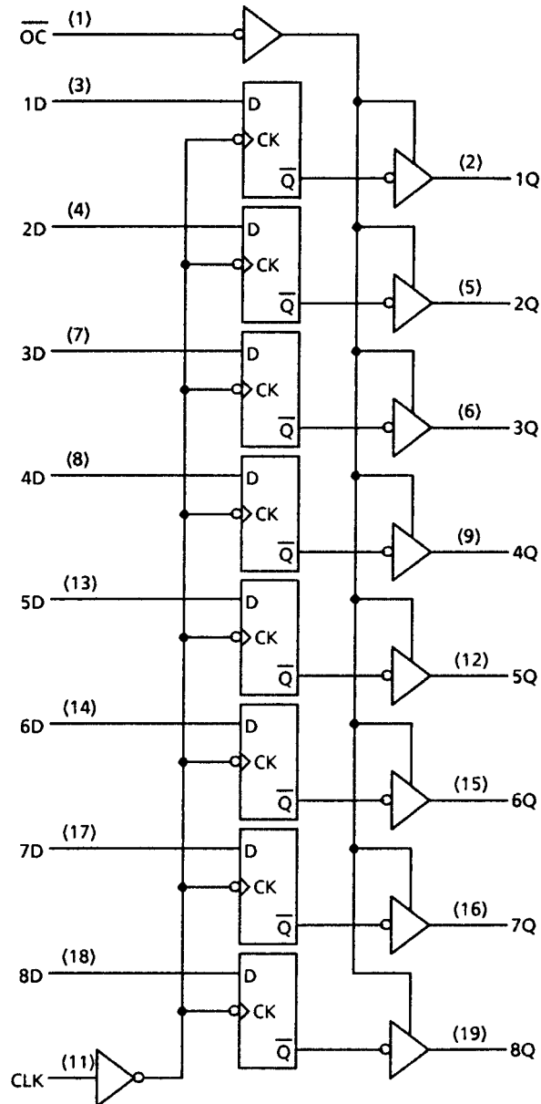
Figure 5: Logic Diagram
