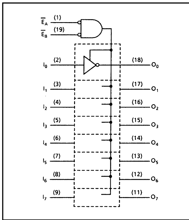
Figure 3: Logic Diagram
