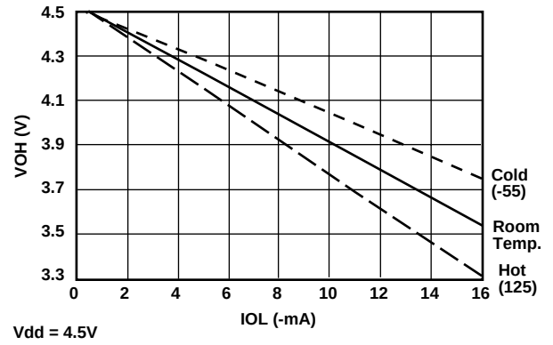
VOH Vs IOH MA9007 Base
