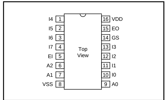
Figure 1: Pin Out
