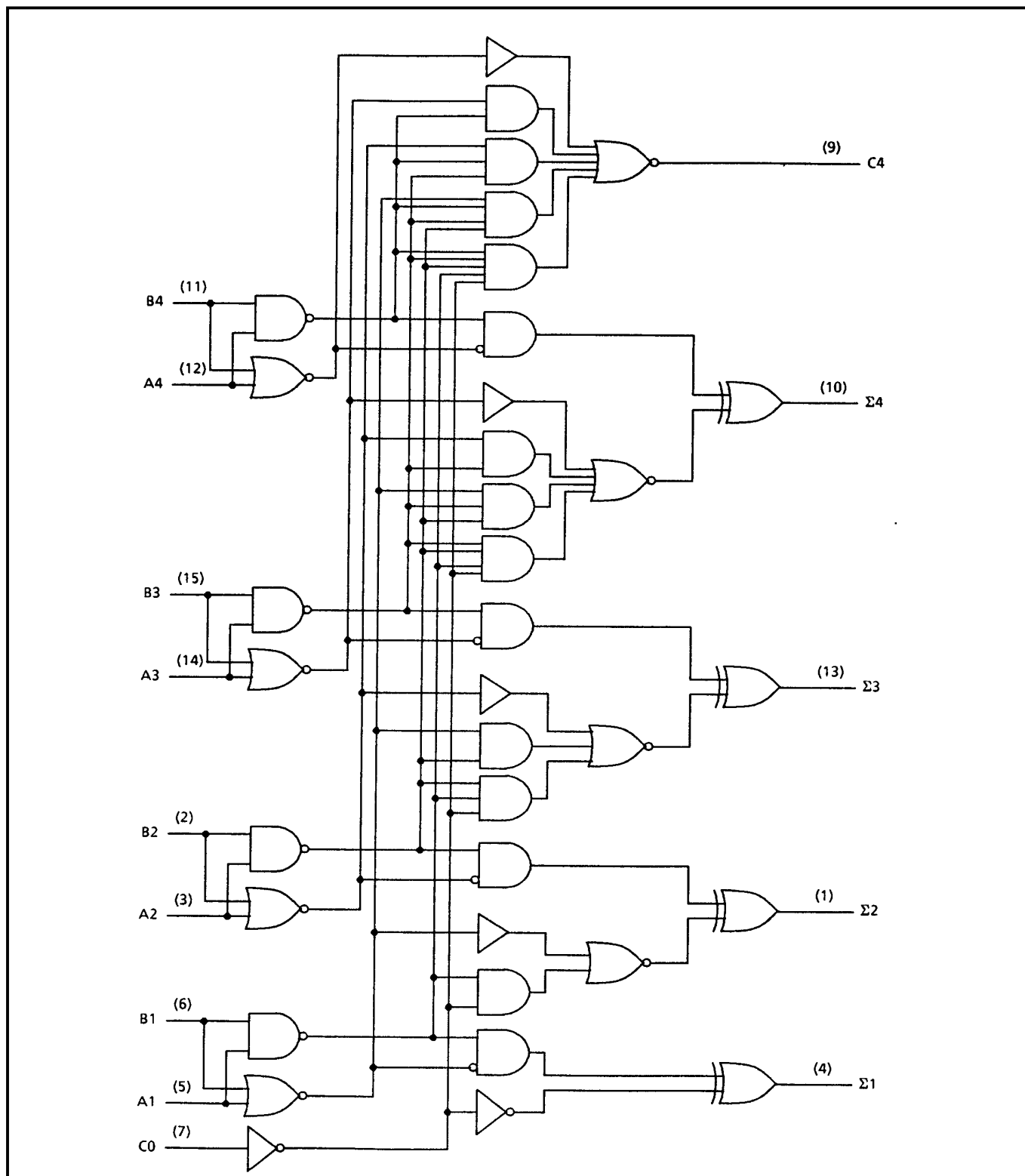
Figure 5: Logic Diagram
