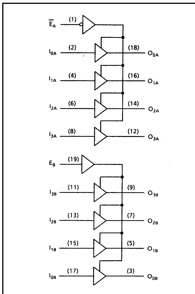
Figure 3: Logic Diagram
