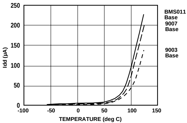
STATIC I dd Vs TEMP.
