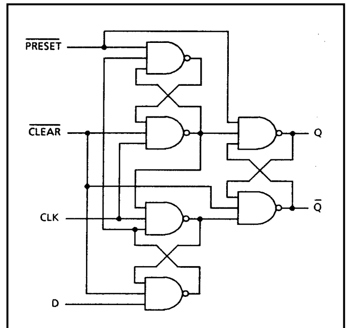
Figure 2: Logic Diagram
