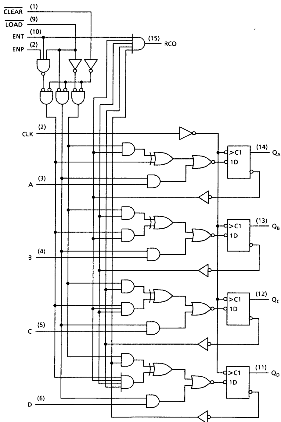
Figure 5: Logic Diagram
