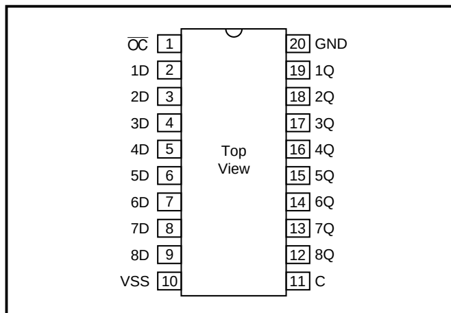
Figure 2: Pin Out
