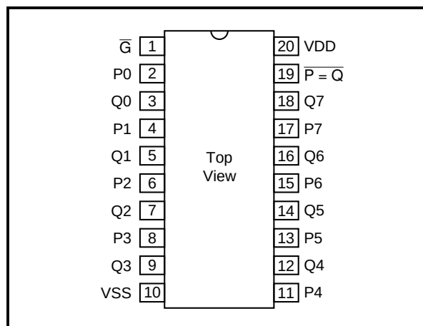
Figure 2: Pin Out
