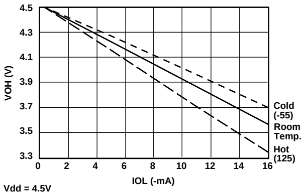
VOH Vs IOH BMS011 Base
