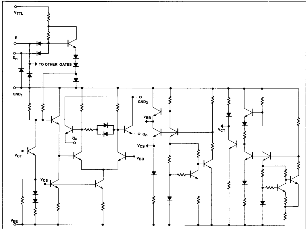
SIMPLIFIED SCHEMATIC
