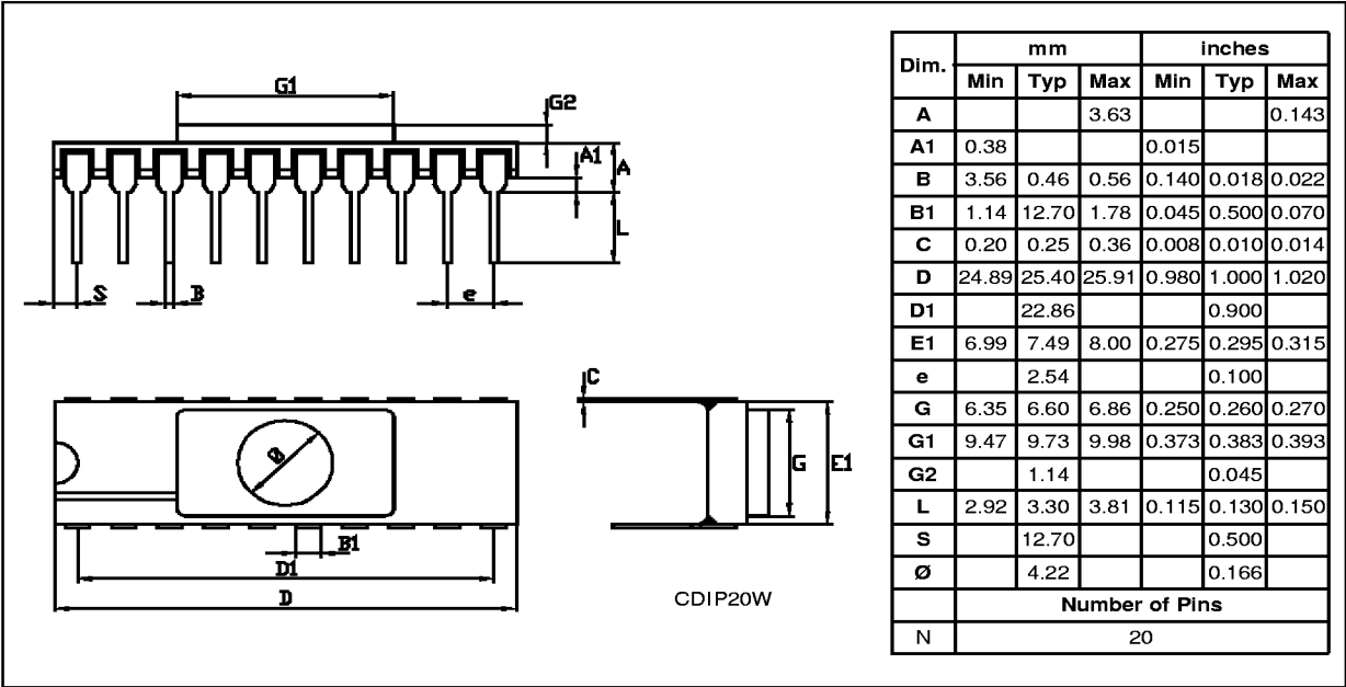
Figure 49. 20-Pin Ceramic Side-Brazed Dual In-Line Package
