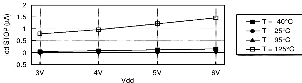
Figure 39. I_{dd\ STOP} versus V_{cc} for ROM devices
