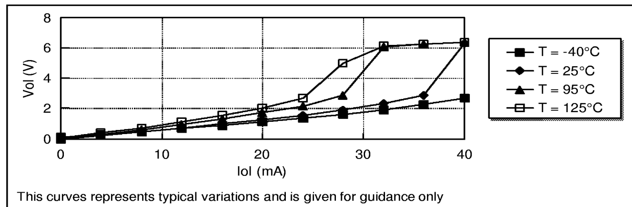
Figure 42. Vol versus Iol on all I/O port at Vdd=5V
