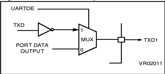
Figure 32. UART Data Output
