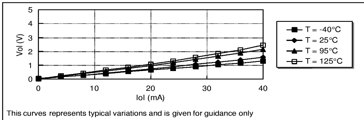
Figure 45. Vol versus Iol for High sink (20mA) I/O ports at Vdd=5V
