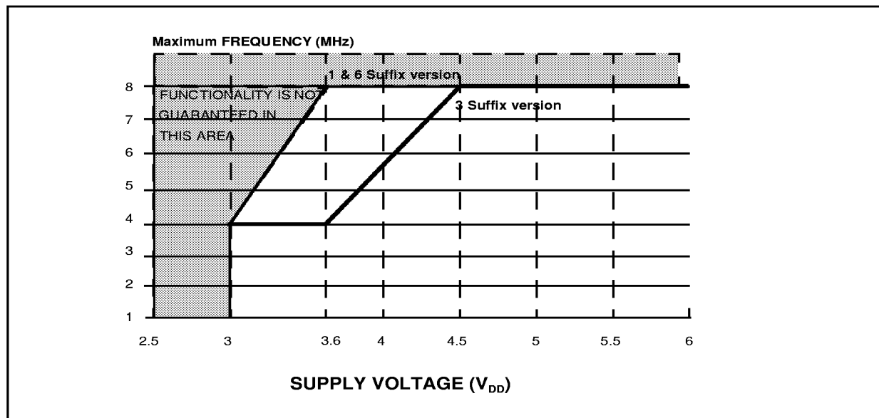
Figure 34. Maximum Operating FREQUENCY (Fmax) Versus SUPPLY VOLTAGE ( V_{DD} )
