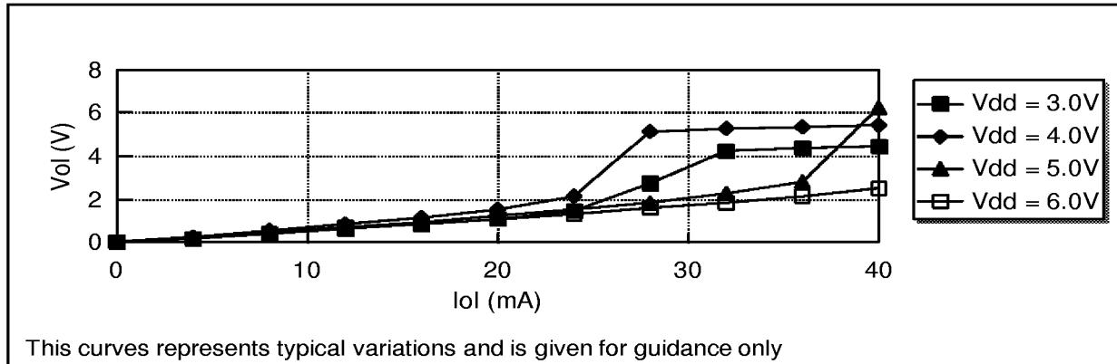
Figure 44. Vol versus Iol for High sink (20mA) I/O ports at T=25°C
