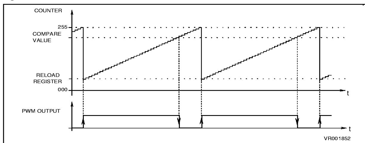
Figure 28. Auto-reload Timer PWM Function
