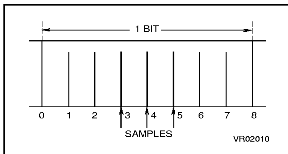
Figure 33. Data Sampling Points
