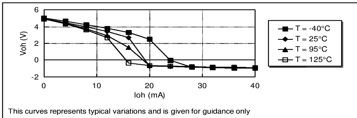
Figure 47. Voh versus loh on all I/O port at Vdd=5V
