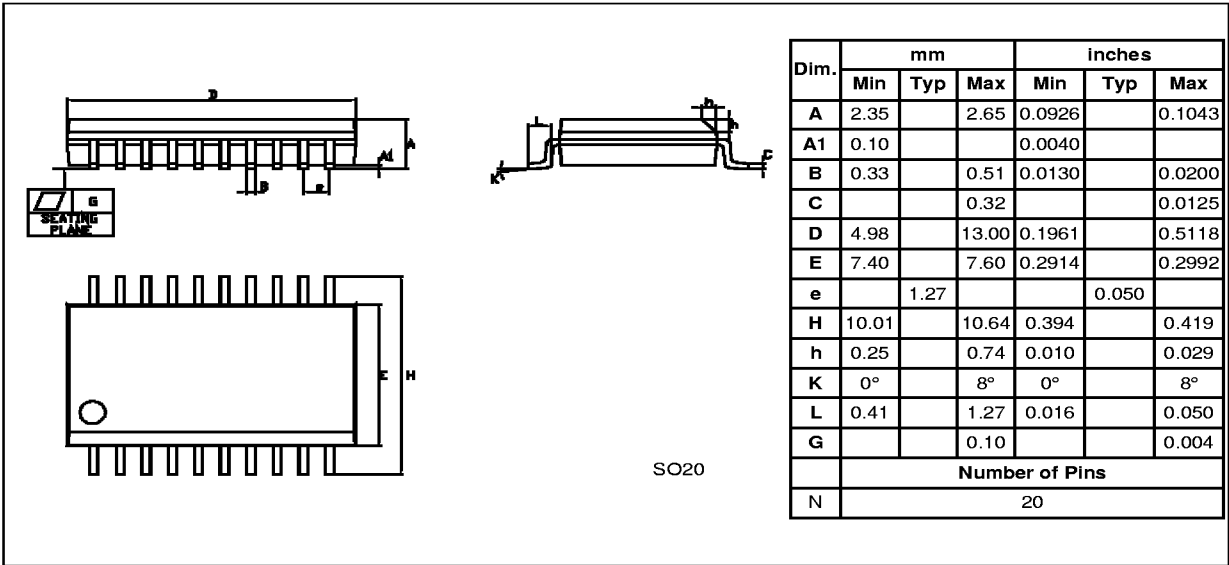
Figure 50. 20-Pin Plastic Small Outline Package, 300-mil Width
