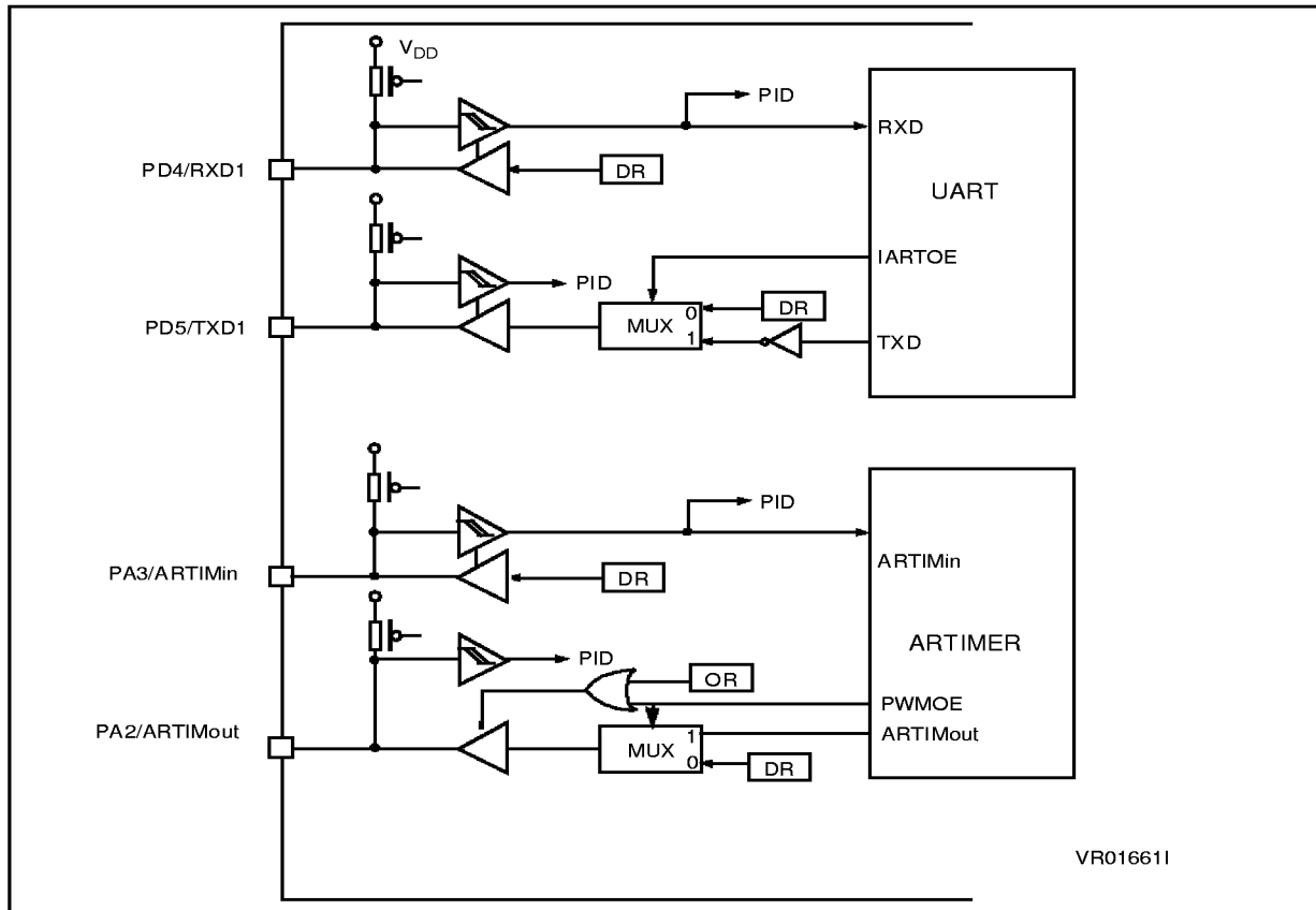
Figure 24. Peripheral Interface Configuration of UART and AR Timer
