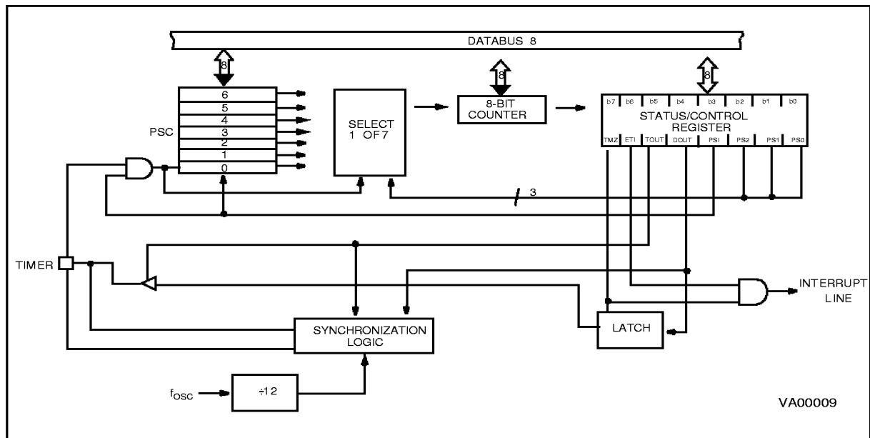
Figure 25. Timer Block Diagram
