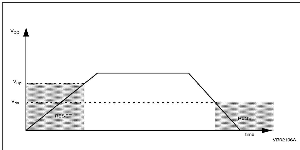
Figure 14. LVD Reset on Power-on and Power-down (Brown-out)
