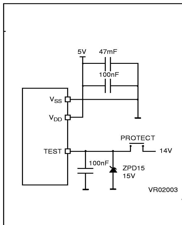
Figure 1. Programming Circuit
