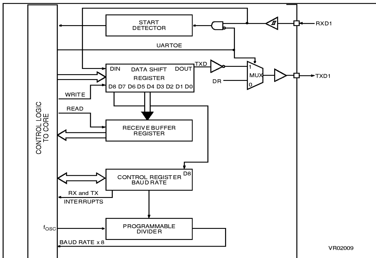
Figure 30. UART Block Diagram
