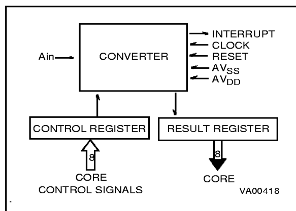
Figure 29. ADC Block Diagram
