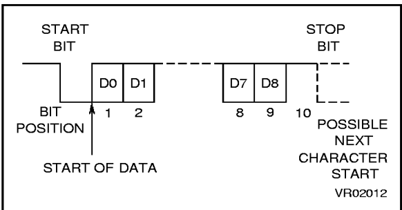
Figure 31. 11-bit Character Format Example
