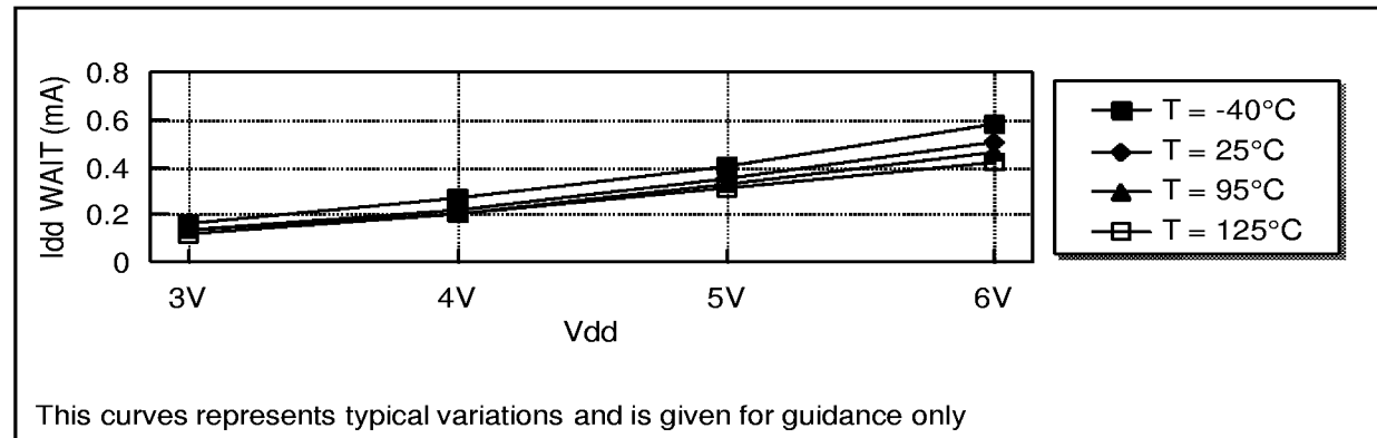
Figure 41. Idd RUN versus Vcc at 8 Mhz for ROM and OTP devices
