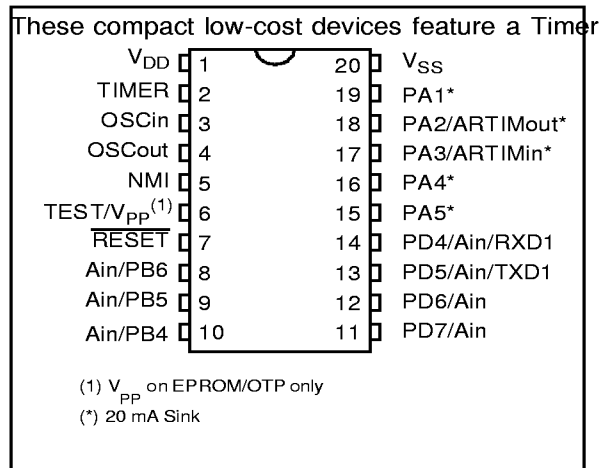
Figure 2. ST62T18C/E18C Pin Configuration
