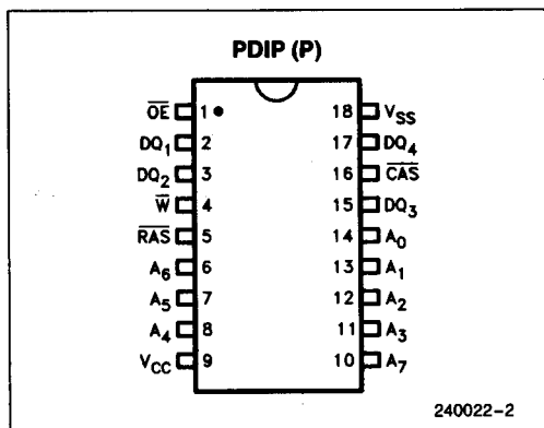
Figure 2. Pin Configuration
