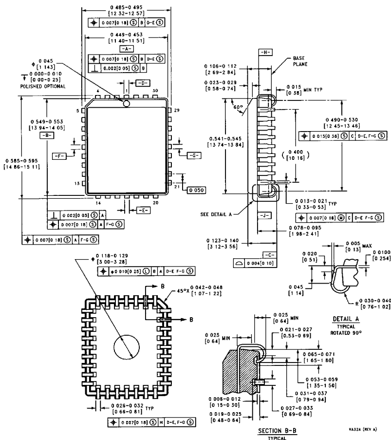
32-Lead PLCC Package (V) Order Number NM27LV020VXXX NS Package Number VA32A
