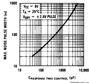
Noise Rejection
