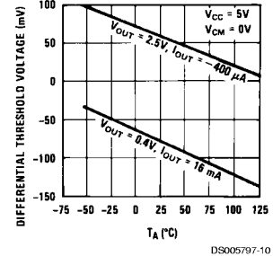
Temperature Sensitivity
