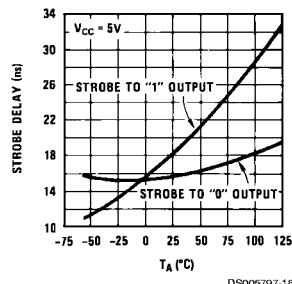
Strobe Delays
